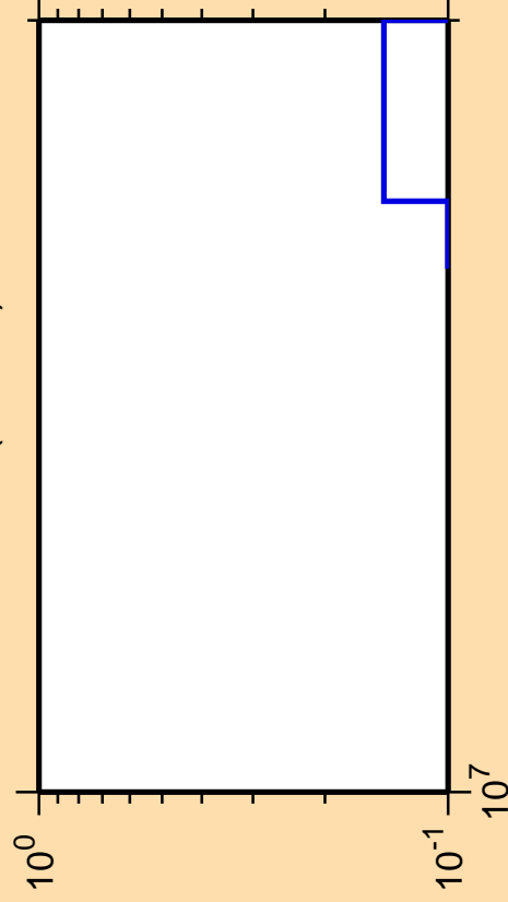
\Delta\sigma/\sigma vs. E for ^{76}\text{Se} (mt117)
