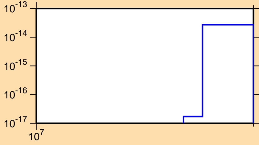
\sigma vs. E for ^{76}\text{Se} (mt117)
