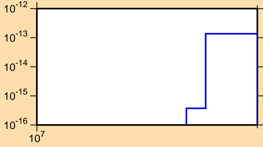
\sigma vs. E for ^{76}\text{Se}(n,2n\alpha)
