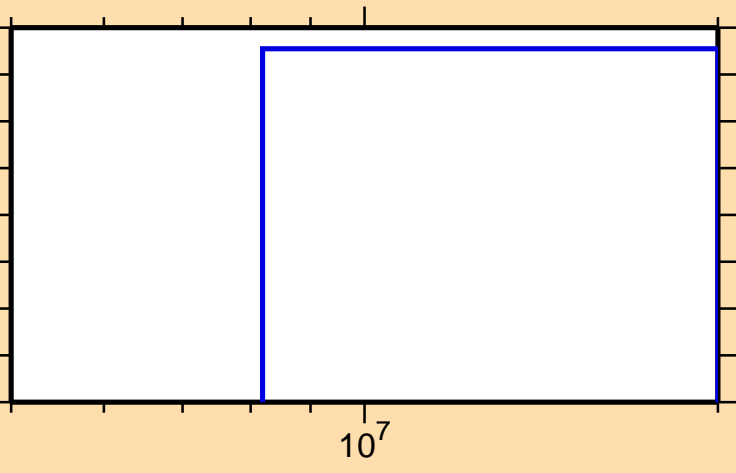
\sigma vs. E for ^{76}\text{Se}(n,np)
