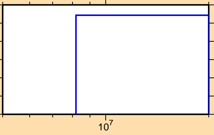
\sigma vs. E for ^{76}\text{Se}(n,3n)
