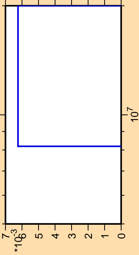
\Delta\sigma/\sigma vs. E for ^{76}\text{Se}(n,2n\alpha)
