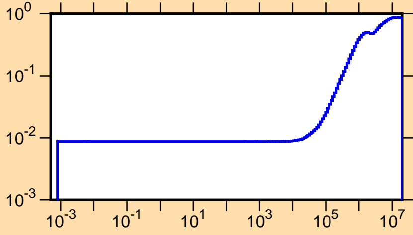
\mu vs. E for ^{77}\text{Se}(\text{mt251})
