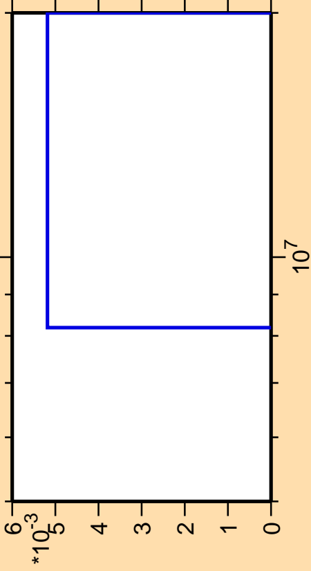
\Delta\sigma/\sigma vs. E for ^{77}\text{Se}(n,\text{pd})
