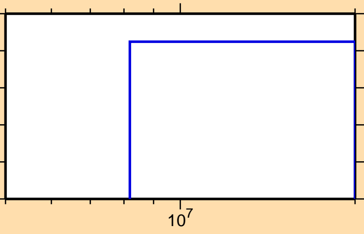
\sigma vs. E for ^{77}\text{Se}(n,\text{nd})
