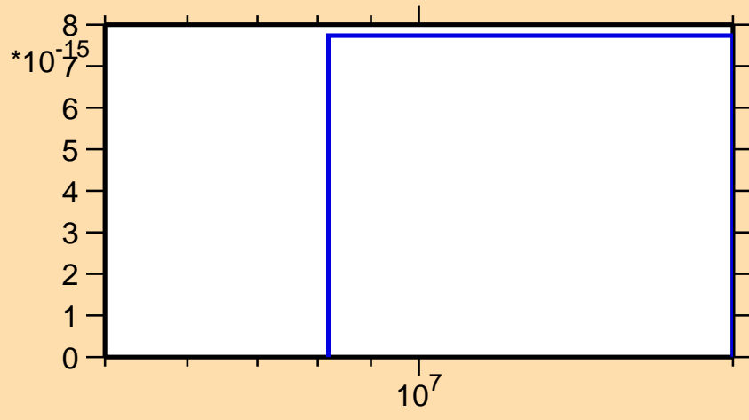
\sigma vs. E for ^{77}\text{Se}(n,\text{pd})
