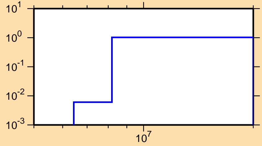
\sigma vs. E for ^{77}\text{Se}(n,2n)
