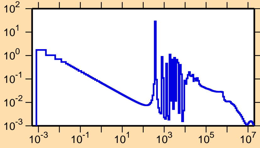
\sigma vs. E for ^{78}\text{Se}(n,\gamma)
