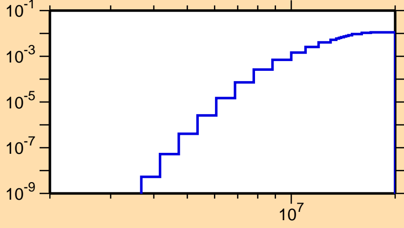
\sigma vs. E for ^{78}\text{Se}(n,\alpha)
