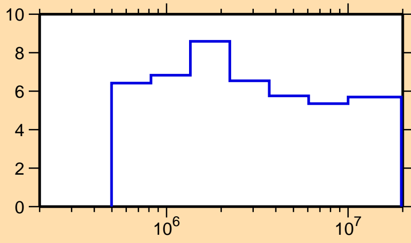
\Delta\sigma/\sigma vs. E for ^{78}\text{Se}(n,\text{nonel.})
