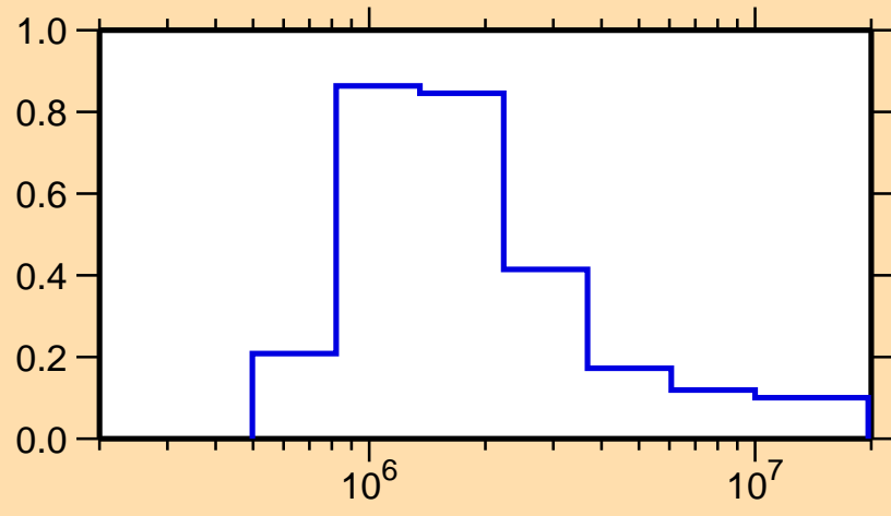
\sigma vs. E for ^{78}\text{Se}(n,n_1)
