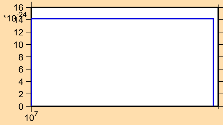
\sigma vs. E for ^{78}\text{Se}(n,\text{pt})
