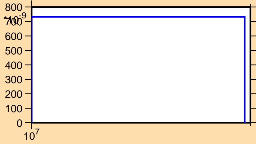
\sigma vs. E for ^{78}\text{Se}(n,t)
