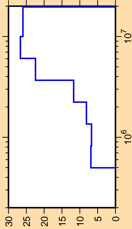
\Delta\sigma/\sigma vs. E for ^{78}\text{Se}(n,n_1)
