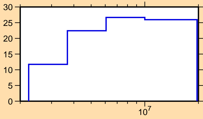
\Delta\sigma/\sigma vs. E for ^{78}\text{Se}(n, n_1)
