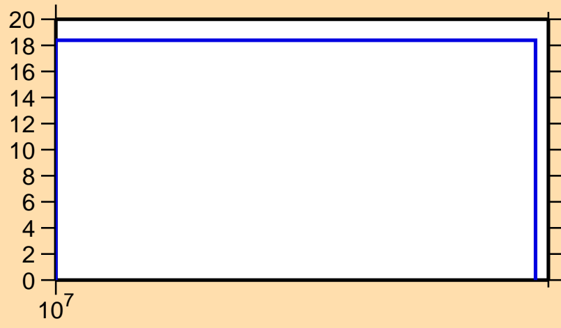
\Delta\sigma/\sigma vs. E for ^{78}\text{Se}(n,\text{inel.})
