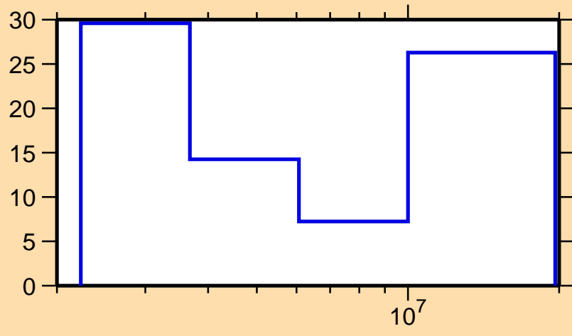
\Delta\sigma/\sigma vs. E for ^{78}\text{Se}(n,n\text{cont.})
