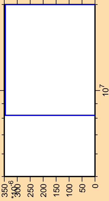
\Delta\sigma/\sigma vs. E for ^{78}\text{Se}(n,pd)
