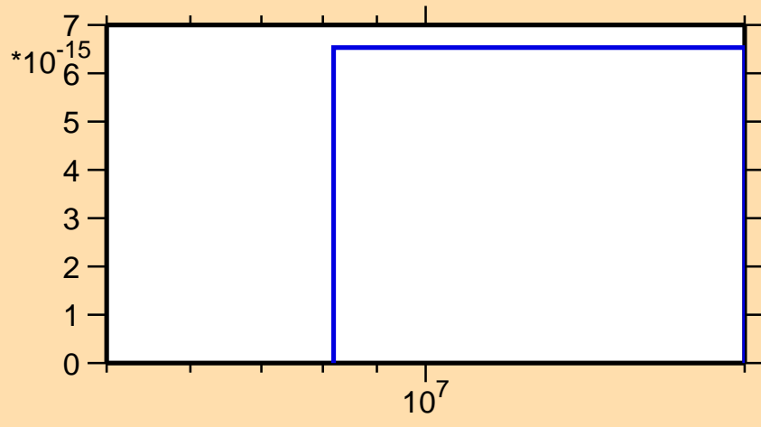
\sigma vs. E for ^{78}\text{Se}(n,p\alpha)
