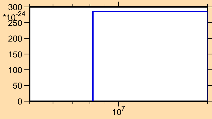
\sigma vs. E for ^{78}\text{Se}(n,nt)
