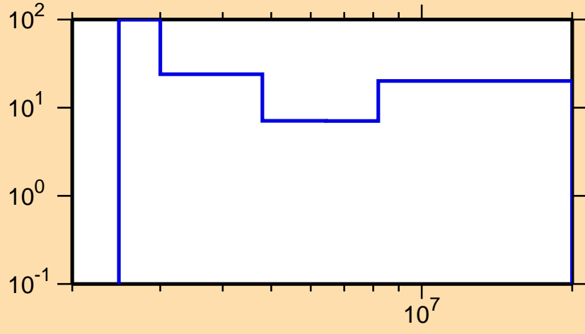
\Delta\sigma/\sigma vs. E for ^{78}\text{Se}(n,n\text{cont.})
