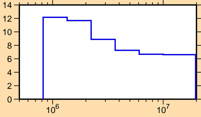
\Delta\sigma/\sigma vs. E for ^{79}\text{Se}(n,n\text{onel.})
