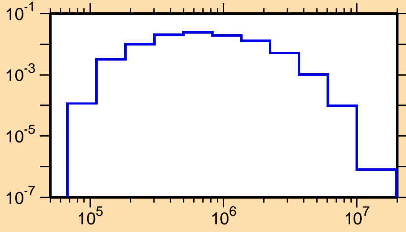
\sigma vs. E for ^{79}\text{Se}(n,n_1)
