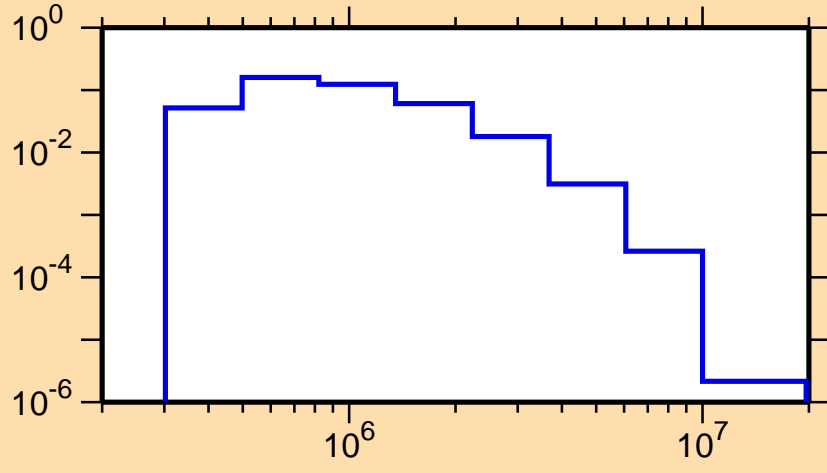
\sigma vs. E for ^{79}\text{Se}(n,n_4)
