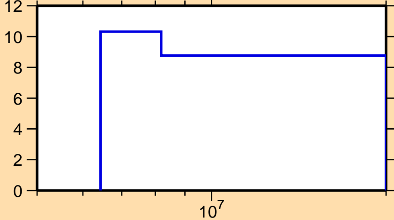
\Delta\sigma/\sigma vs. E for ^{79}\text{Se}(n,\text{nonel.})
