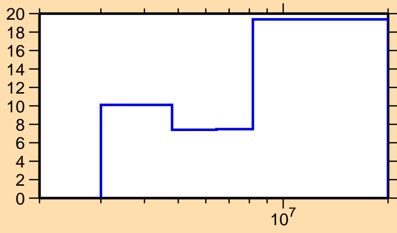
\Delta\sigma/\sigma vs. E for ^{80}\text{Se}(n,n\text{cont.})
