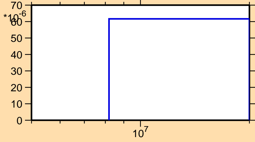
\sigma vs. E for ^{80}\text{Se}(n,n\alpha)
