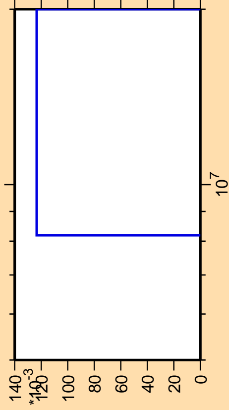
\Delta\sigma/\sigma vs. E for ^{80}\text{Se}(n,\text{nd})
