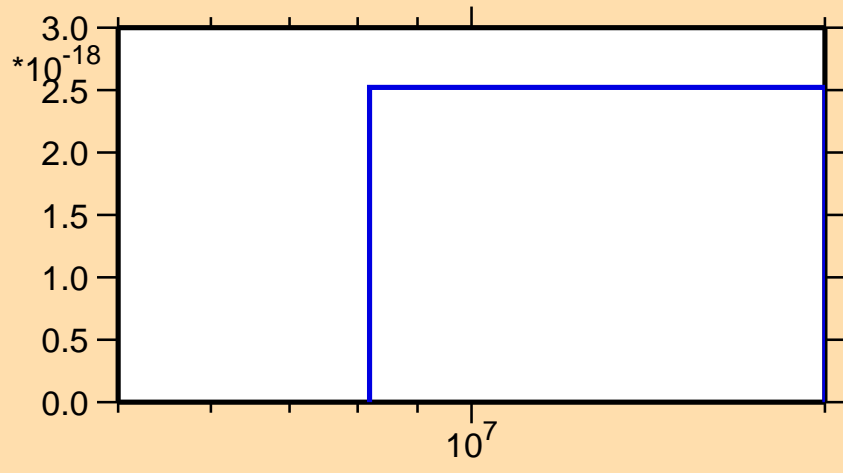
\sigma vs. E for ^{80}\text{Se}(n,2n\alpha)
