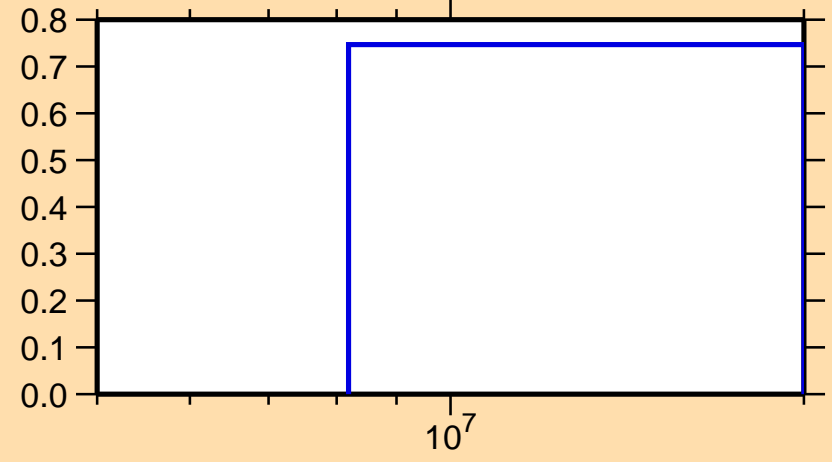
\sigma vs. E for ^{80}\text{Se}(n,2n)
