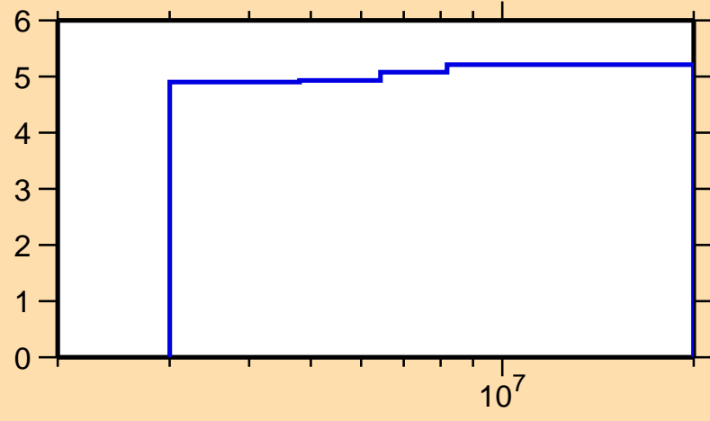
\Delta\sigma/\sigma vs. E for ^{80}\text{Se}(n,n\text{nonel.})
