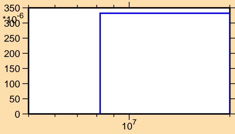
\sigma vs. E for ^{80}\text{Se}(n,d)
