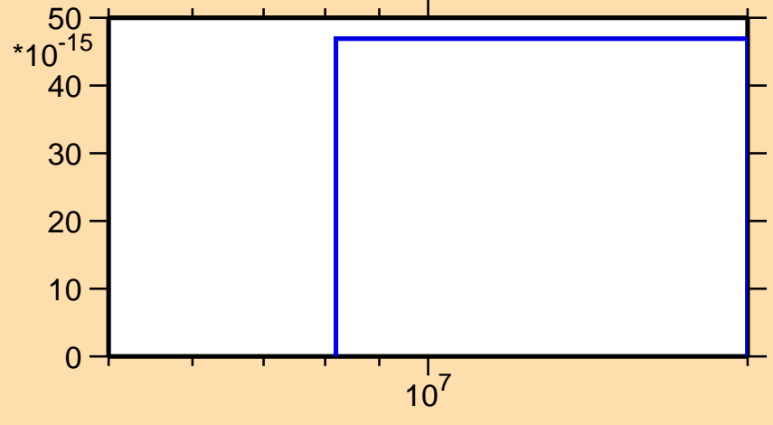
\sigma vs. E for ^{80}\text{Se}(n,\text{nd})
