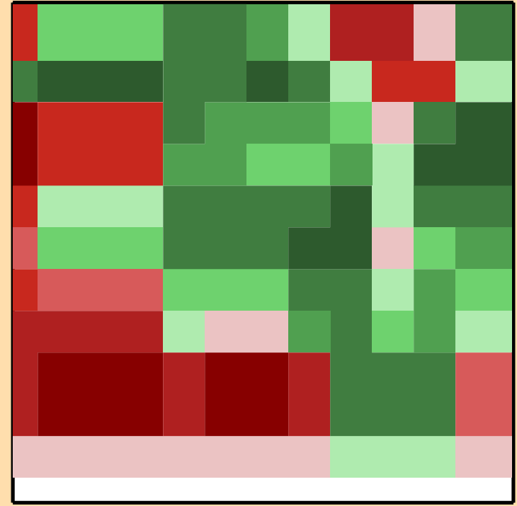
\Delta\sigma/\sigma vs. E for ^{81}\text{Se}(n,\text{tot.})
