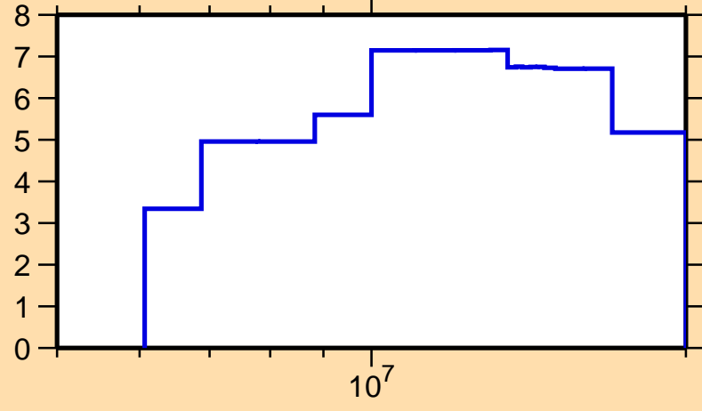
\Delta\sigma/\sigma vs. E for ^{82}\text{Se}(n,tot.)
