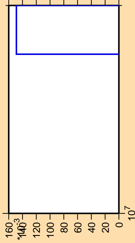
\Delta\sigma/\sigma vs. E for ^{82}\text{Se}(n,\text{nd})
