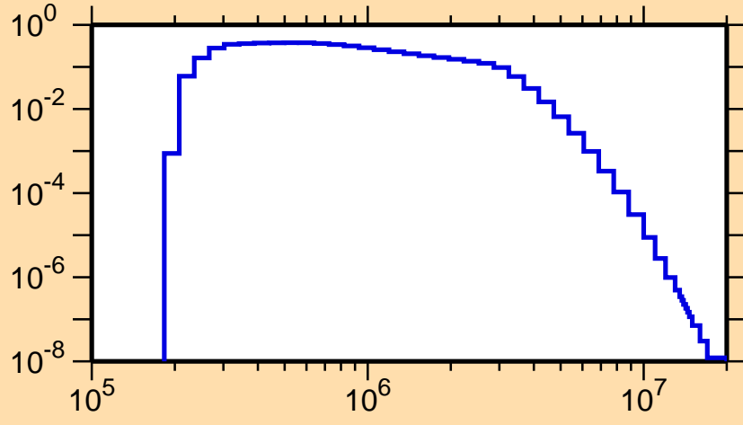
\sigma vs. E for ^{83}\text{Se}(n,n_3)
