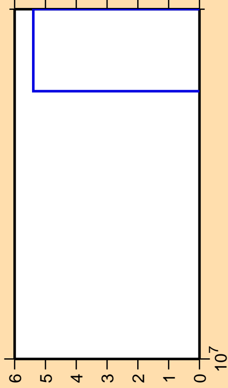
\Delta\sigma/\sigma vs. E for ^{83}\text{Se}(n,nt)
