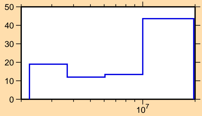
\Delta\sigma/\sigma vs. E for ^{83}\text{Se}(n,n\text{cont.})
