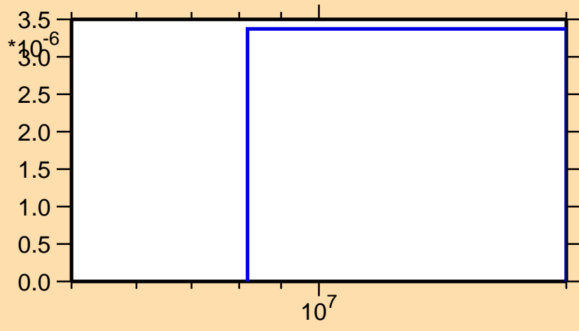
\sigma vs. E for ^{83}\text{Se}(n,n\alpha)
