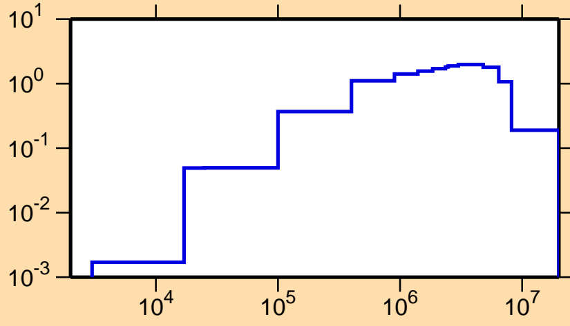
\sigma vs. E for ^{83}\text{Se}(n,\text{inel.})
