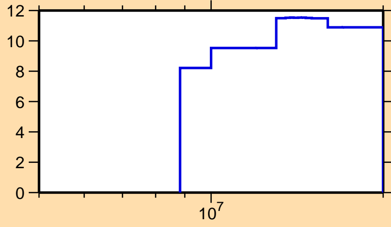
\Delta\sigma/\sigma vs. E for ^{84}\text{Se}(n,el.)
