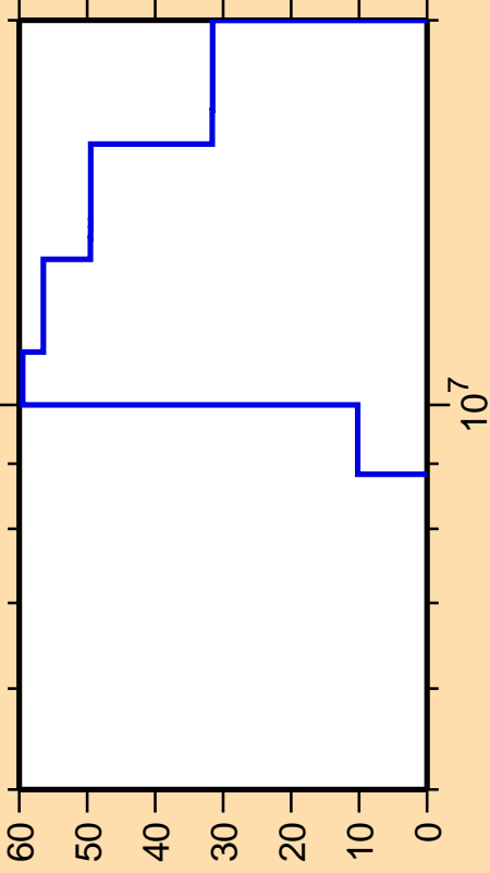
\Delta\sigma/\sigma vs. E for ^{84}\text{Se}(n,p)
