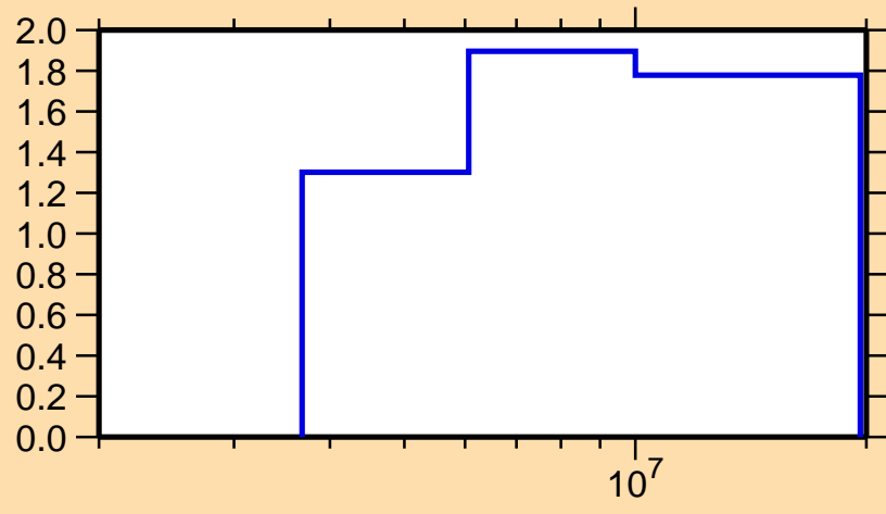
\Delta\sigma/\sigma vs. E for ^{84}\text{Se}(n,n\text{onrel.})
