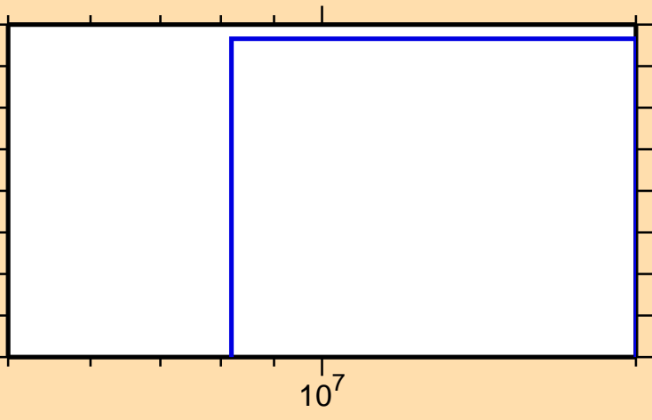
\sigma vs. E for ^{84}\text{Se}(n,d)
