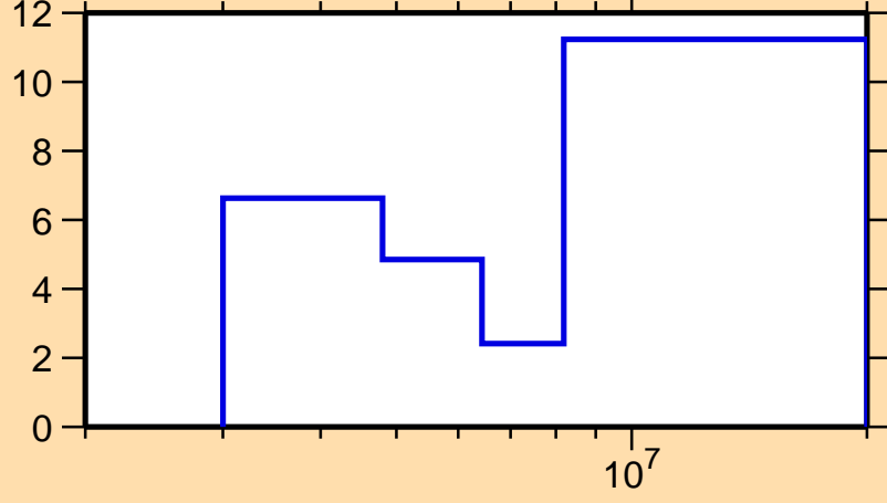
Delta sigma/sigma vs. E for 84 Se(n,ncont.)
