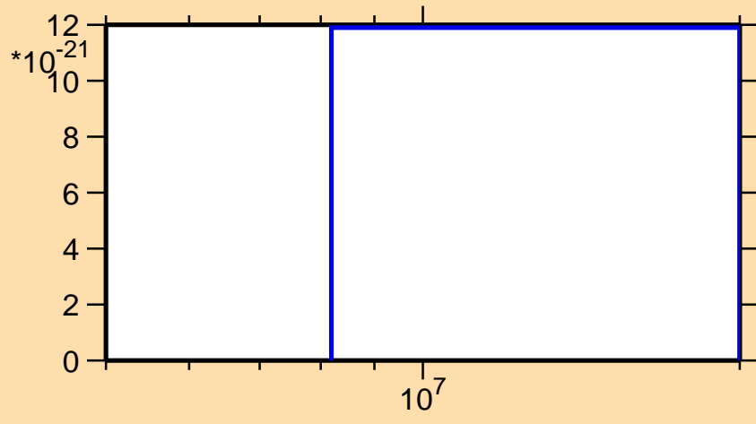
\sigma vs. E for ^{84}\text{Se}(n,nd)
