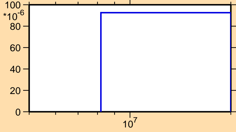
\sigma vs. E for ^{84}\text{Se}(n,p)
