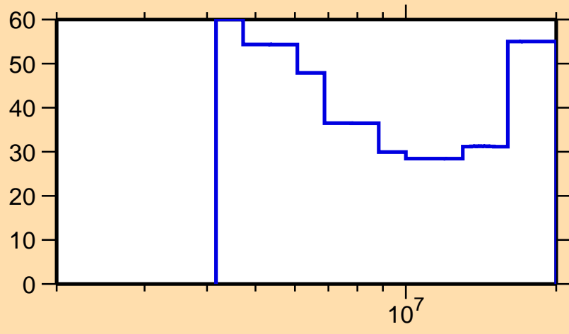
\Delta\sigma/\sigma vs. E for ^{85}\text{Se}(n,2n)
