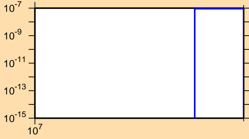
\sigma vs. E for ^{85}\text{Se}(n,nd)
