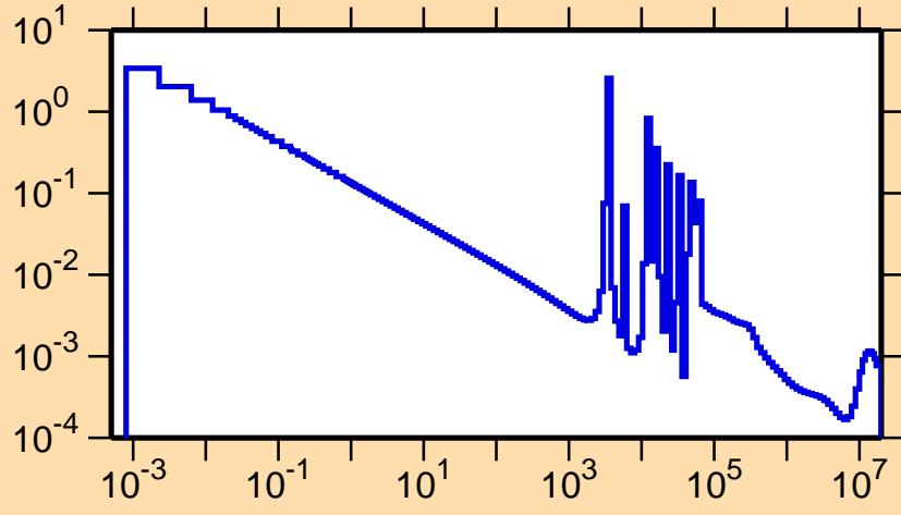
\sigma vs. E for ^{85}\text{Se}(n,\gamma)
