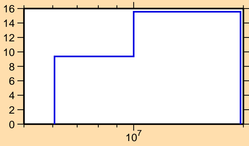
\Delta\sigma/\sigma vs. E for ^{85}\text{Se}(n,el.)
