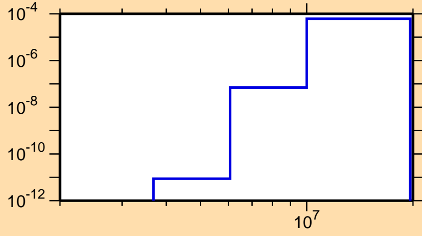
\sigma vs. E for ^{85}\text{Se}(n,\alpha)
