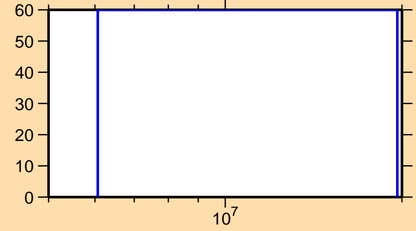
\Delta\sigma/\sigma vs. E for ^{85}\text{Se}(n,\gamma)
