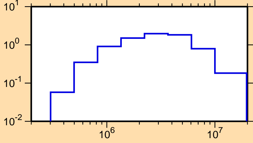
\sigma vs. E for ^{85}\text{Se}(n,\text{inel.})
