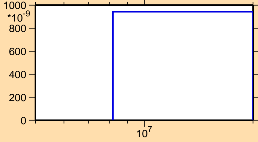
\sigma vs. E for ^{85}\text{Se}(n,n\alpha)
