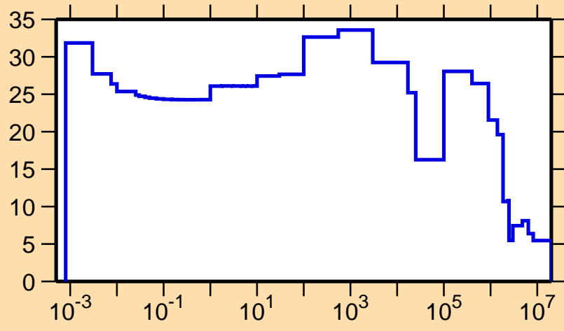
\Delta\sigma/\sigma vs. E for ^{85}\text{Se}(n,\text{tot.})
