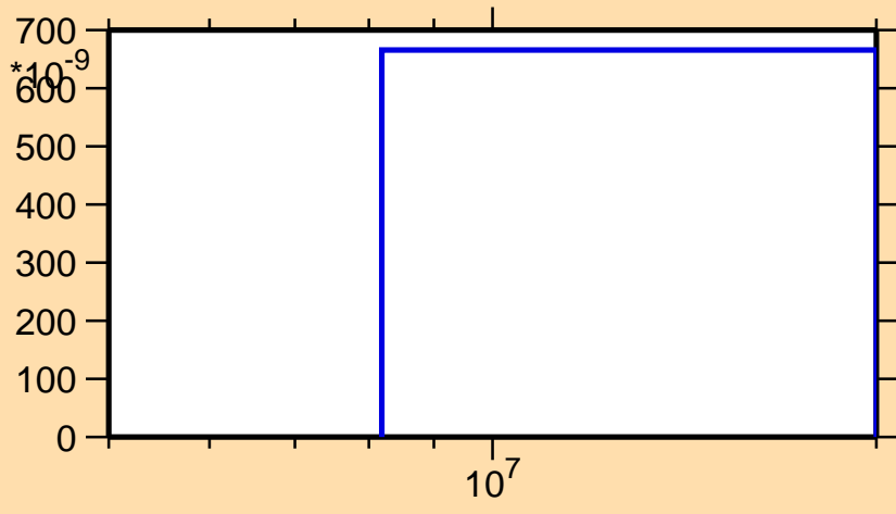
\sigma vs. E for ^{85}\text{Se}(n,np)
