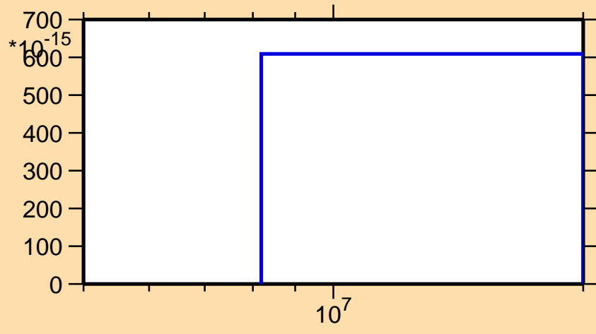
\sigma vs. E for ^{85}\text{Se}(n,nt)
