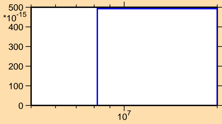
\sigma vs. E for ^{85}\text{Se}(n,2n\alpha)
