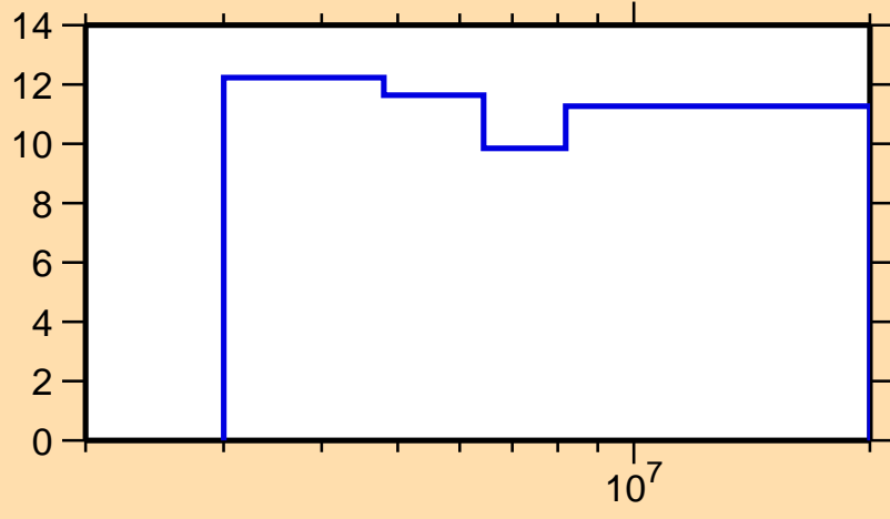
\Delta\sigma/\sigma vs. E for ^{85}\text{Se}(n,\text{nonel.})
