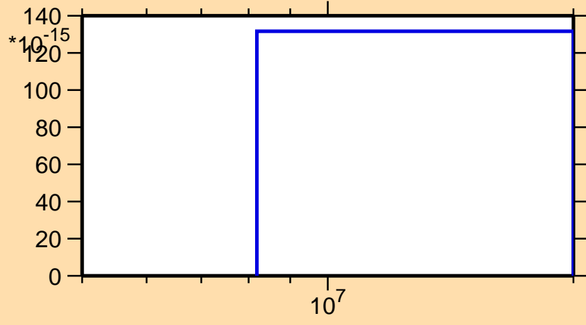
\sigma vs. E for ^{85}\text{Se}(n,2np)
