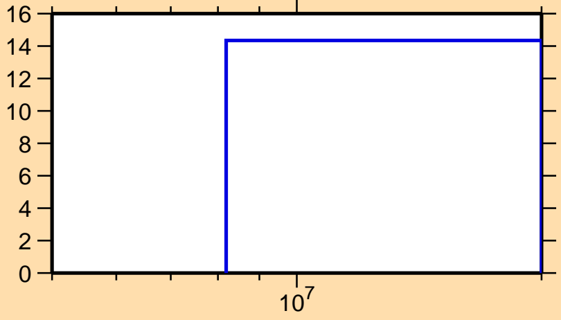
\Delta\sigma/\sigma vs. E for ^{85}\text{Se}(n,el.)
