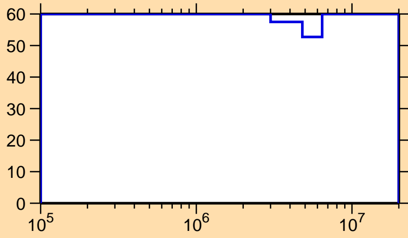
\Delta\sigma/\sigma vs. E for ^{85}\text{Se}(n,n_1)
