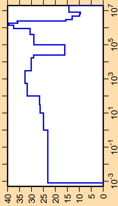
\Delta\sigma/\sigma vs. E for ^{85}\text{Se}(n,\text{el.})
