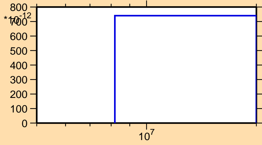
\sigma vs. E for ^{85}\text{Se}(n,nd)
