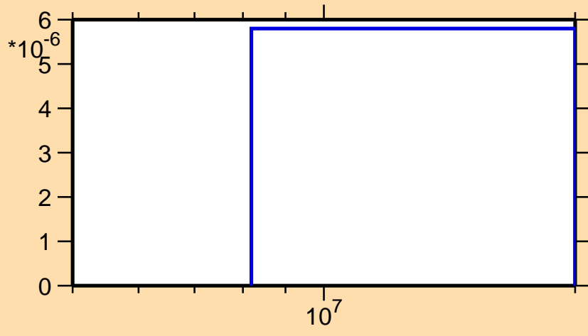
\sigma vs. E for ^{85}\text{Se}(n,t)
