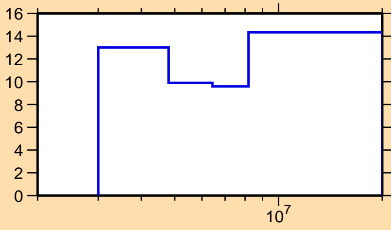
\Delta\sigma/\sigma vs. E for ^{85}\text{Se}(n,\text{el.})
