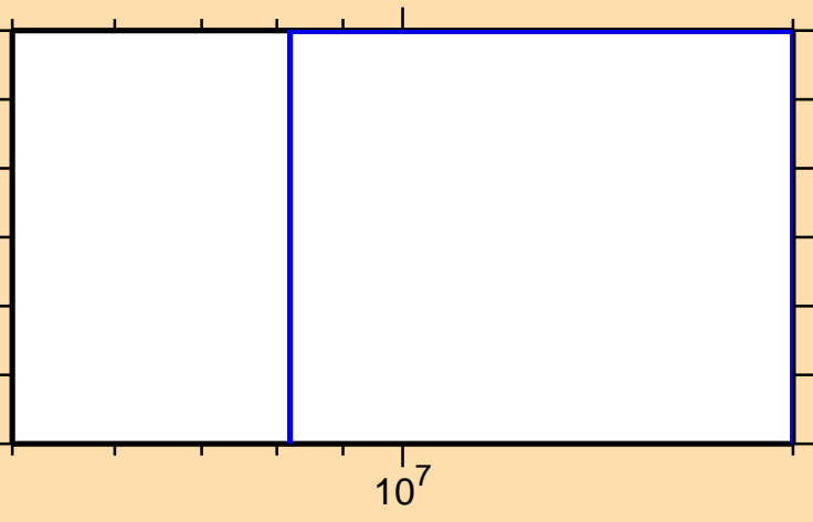
\sigma vs. E for ^{85}\text{Se}(n,3n)
