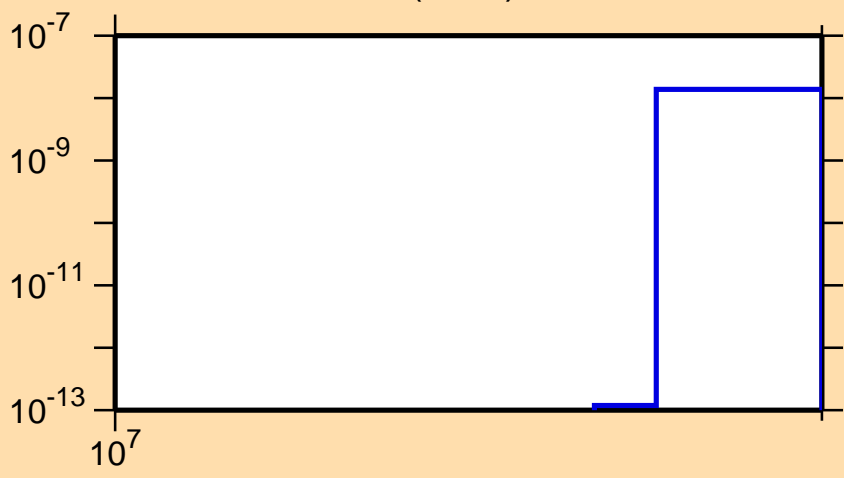
\sigma vs. E for ^{87}\text{Se}(n,\text{nd})
