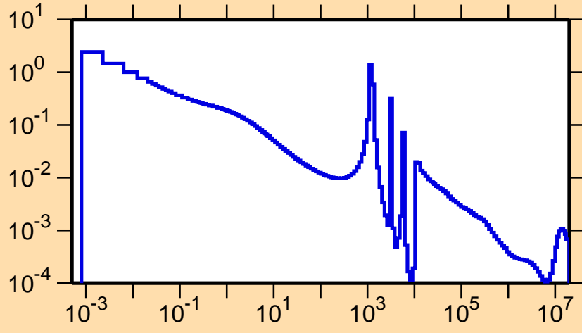
\sigma vs. E for ^{87}\text{Se}(n,\gamma)
