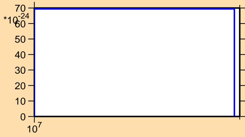
\sigma vs. E for ^{87}\text{Se}(n,3n\alpha)
