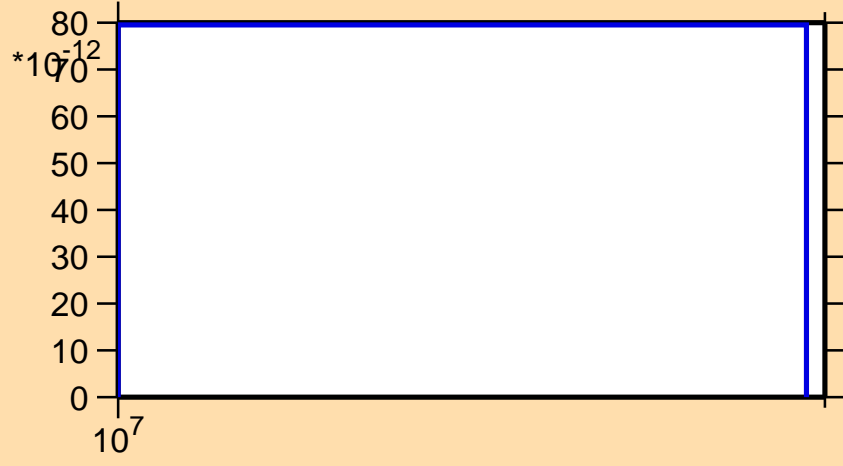
\sigma vs. E for ^{87}\text{Se}(n,nd)
