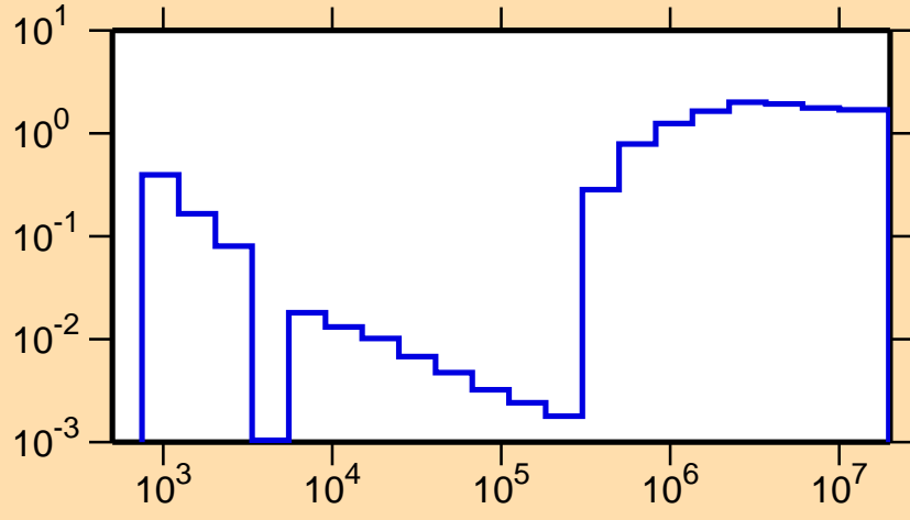
\sigma vs. E for ^{87}\text{Se}(n,\text{nonel.})
