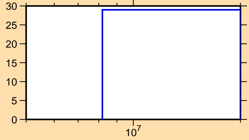
\Delta\sigma/\sigma vs. E for ^{87}\text{Se}(n,el.)
