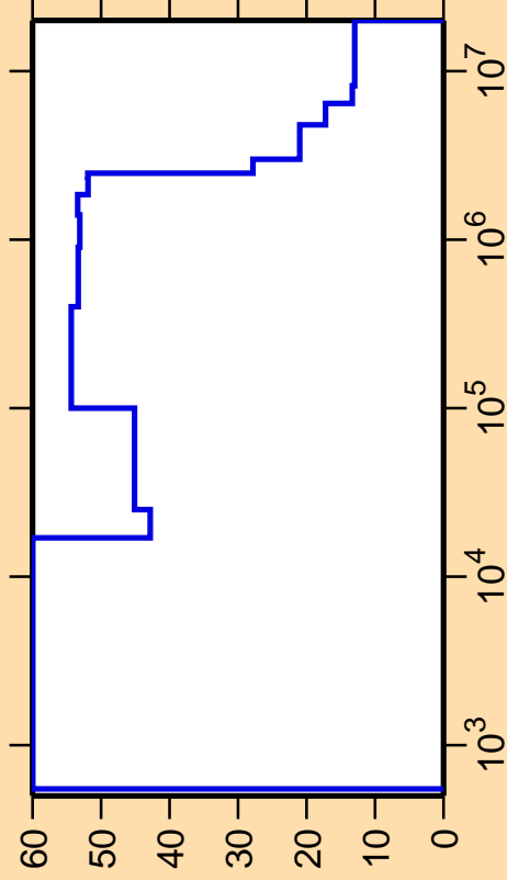
\Delta\sigma/\sigma vs. E for ^{87}\text{Se}(n,\text{nonel.})
