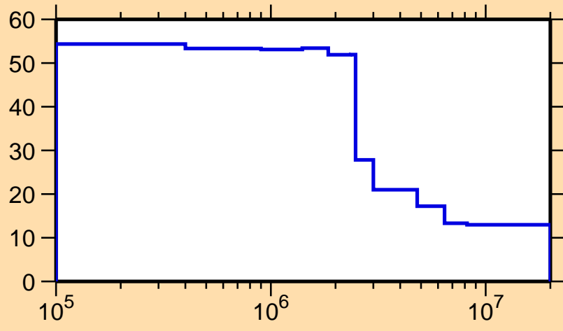
\Delta\sigma/\sigma vs. E for ^{87}\text{Se}(n,n\text{onel.})
