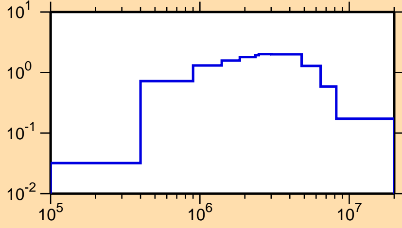
\sigma vs. E for ^{87}\text{Se}(n,\text{inel.})
