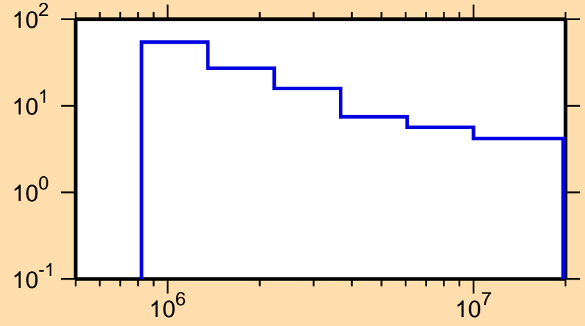
\Delta\sigma/\sigma vs. E for ^{88}\text{Se}(n,\text{nonel.})
