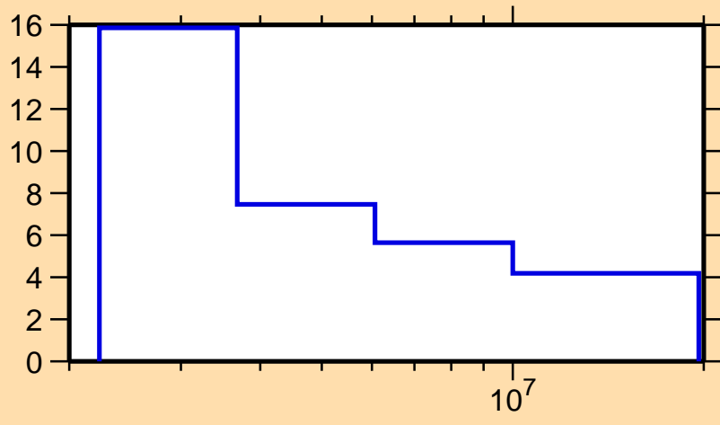
\Delta\sigma/\sigma vs. E for ^{88}\text{Se}(n,n\text{onel.})
