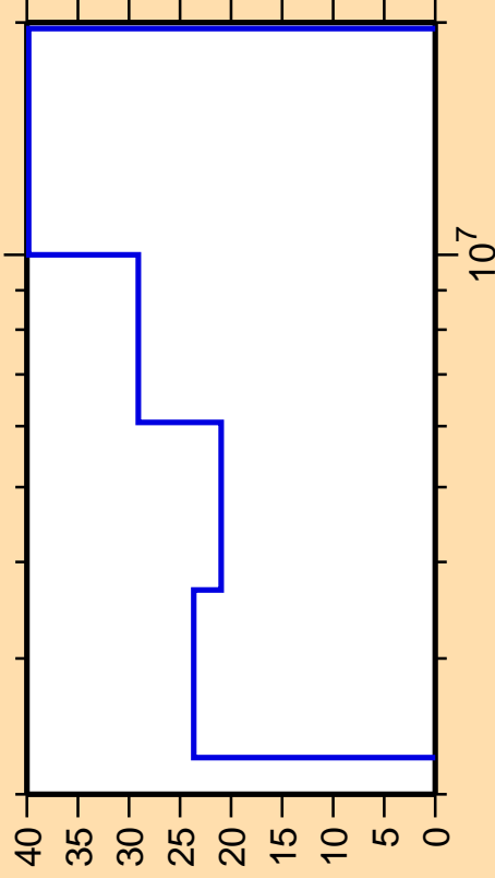
\Delta\sigma/\sigma vs. E for ^{88}\text{Se}(n,n\text{cont.})
