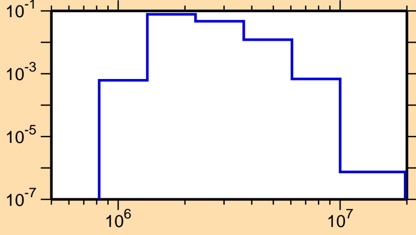
\sigma vs. E for ^{88}\text{Se}(n,n_3)
