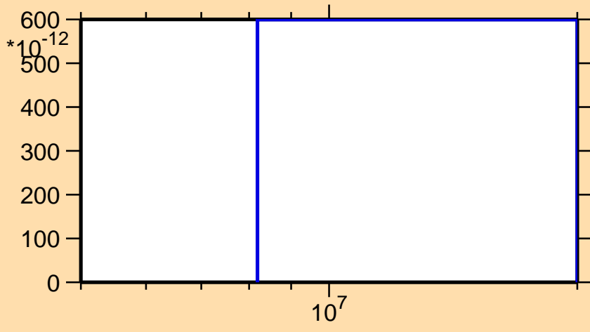
\sigma vs. E for ^{267}\text{Lu}
