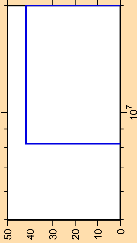
\Delta\sigma/\sigma vs. E for ^{27}\text{Si}(n,n\text{cont.})
