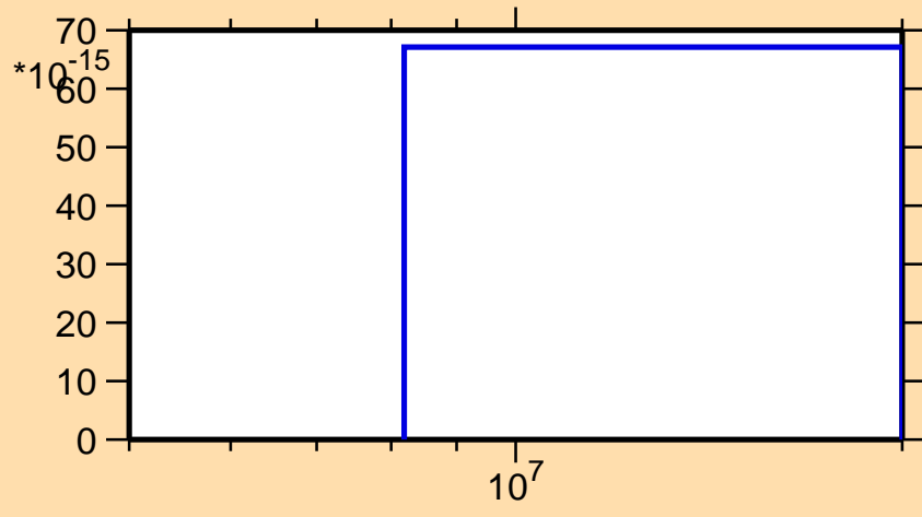
\sigma vs. E for ^{27}\text{Si} (mt 45)
