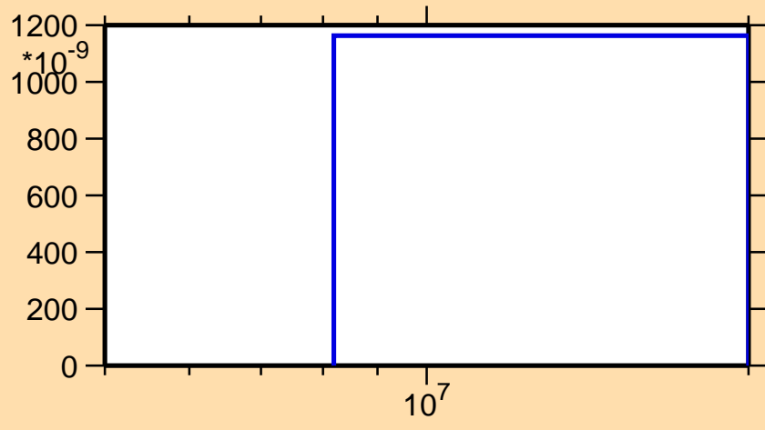
\sigma vs. E for ^{27}\text{Si}(\text{mt } 34)
