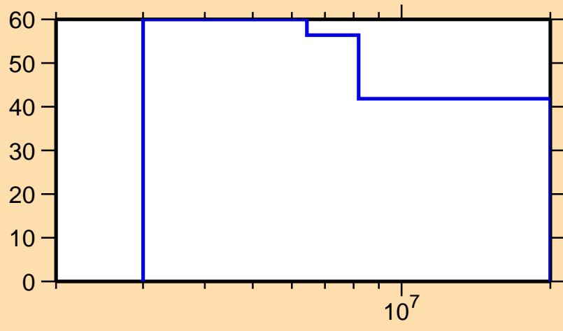
\Delta\sigma/\sigma vs. E for ^{27}\text{Si}(n,ncont.)
