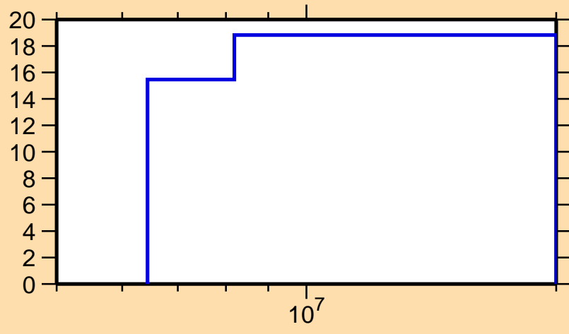
\Delta\sigma/\sigma vs. E for ^{29}\text{Si}(n,n\text{cont.})
