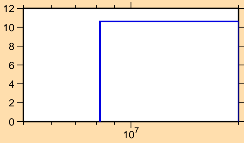
\Delta\sigma/\sigma vs. E for ^{29}\text{Si}(n,2n)
