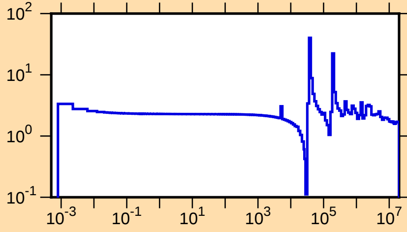
\sigma vs. E for ^{30}\text{Si}(n,\text{tot.})
