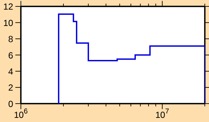
\Delta\sigma/\sigma vs. E for ^{30}\text{Si}(\text{n},\text{nonel.})
