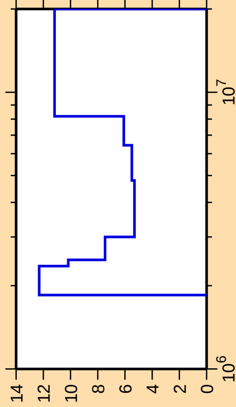
\Delta\sigma/\sigma vs. E for ^{30}\text{Si}(\text{n},\text{inel.})
