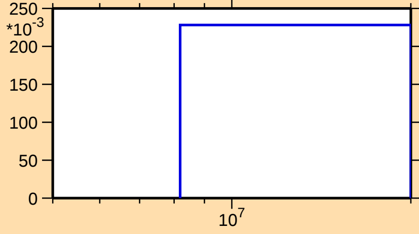
\sigma vs. E for ^{30}\text{Si}(n,2n)
