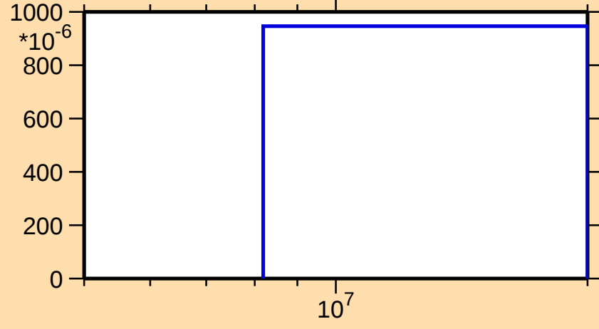
\sigma vs. E for ^{30}\text{Si}(n,d)
