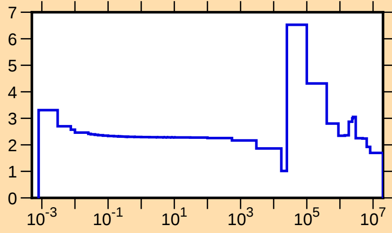
\sigma vs. E for ^{30}\text{Si}(n,\text{tot.})
