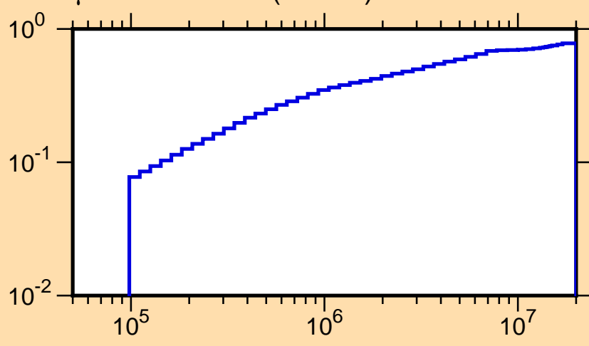
\mu vs. E for ^{31}\text{Si}(\text{mt251})
