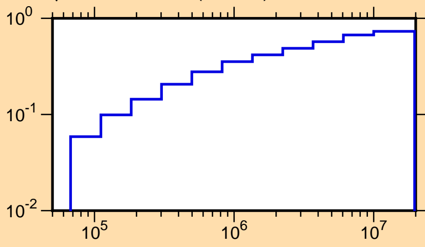
\mu vs. E for ^{31}\text{Si}(\text{mt251})
