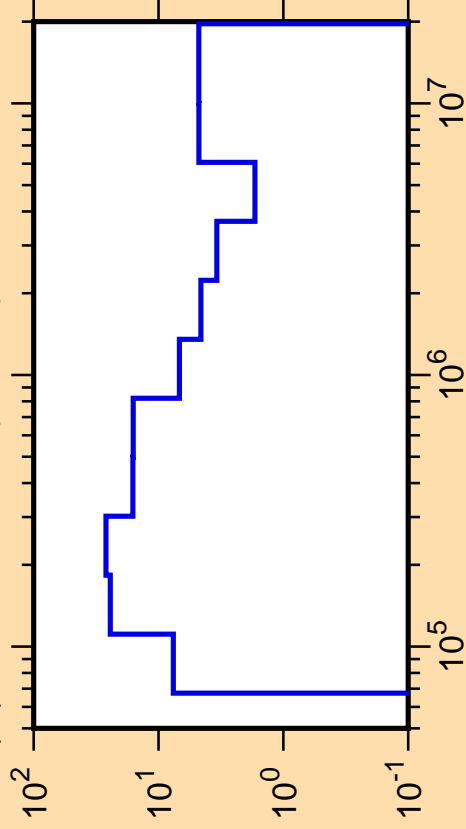
\Delta\mu/\mu vs. E for ^{31}\text{Si}(\text{mt251})
