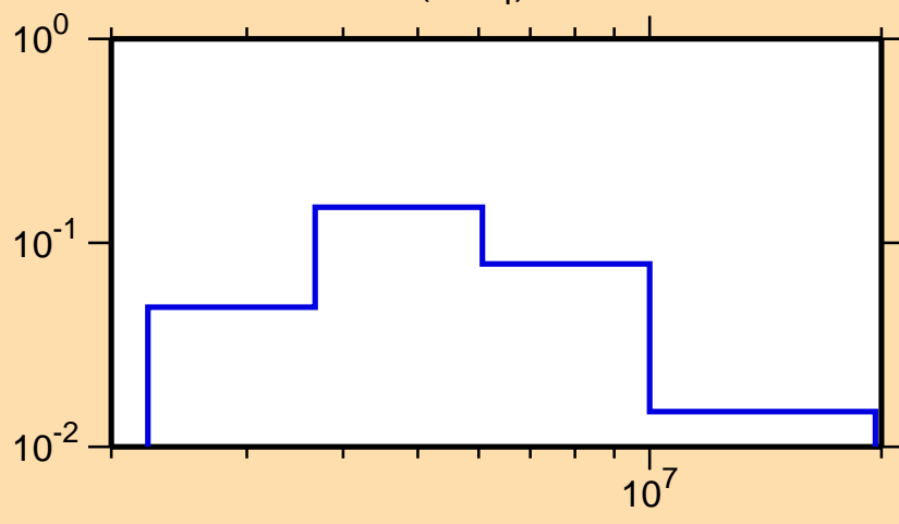
\sigma vs. E for ^{31}\text{Si}(n,n_4)
