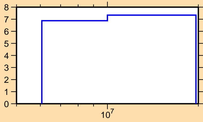
\Delta\sigma/\sigma vs. E for ^{31}\text{Si}(n,n\text{onel.})
