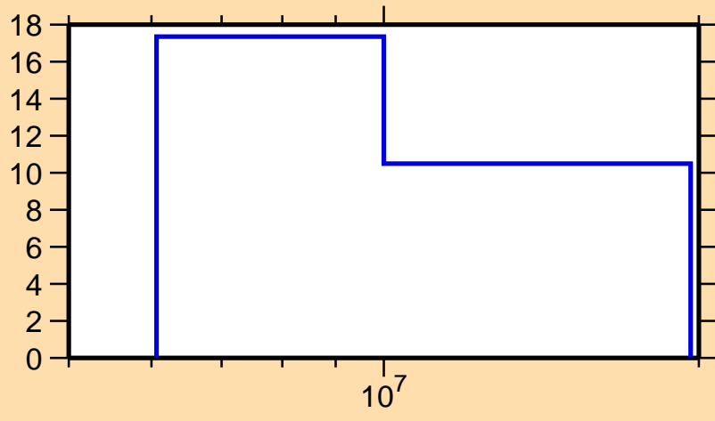
\Delta\sigma/\sigma vs. E for ^{31}\text{Si}(n,2n)
