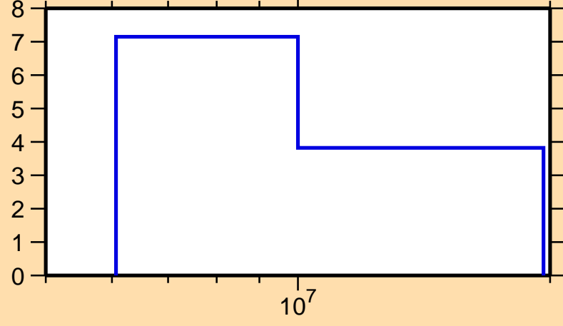
\Delta\sigma/\sigma vs. E for ^{31}\text{Si}(n,\text{tot.})
