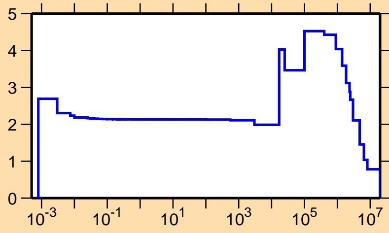
\sigma vs. E for ^{31}\text{Si}(n,\text{el.})
