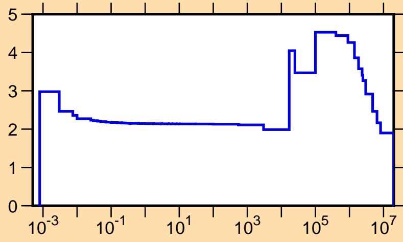
\sigma vs. E for ^{31}\text{Si}(n,\text{tot.})
