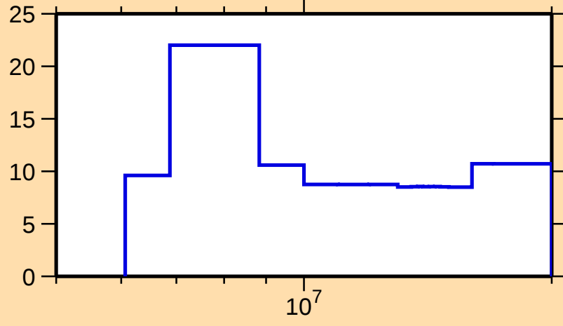
\Delta\sigma/\sigma vs. E for ^{33}\text{Si}(n,2n)
