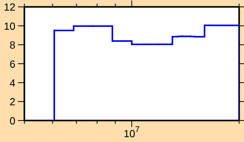
\Delta\sigma/\sigma vs. E for ^{33}\text{Si}(n,n\text{onel.})
