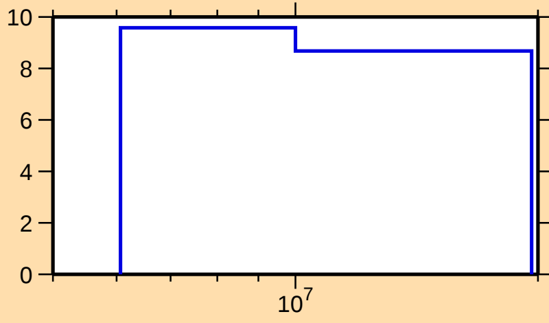
\Delta\sigma/\sigma vs. E for ^{33}\text{Si}(\text{n},\text{nonel.})
