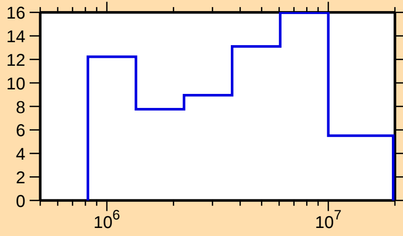
\Delta\sigma/\sigma vs. E for ^{33}\text{Si}(\text{n,el.})
