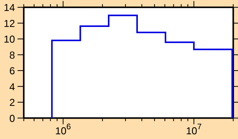
\Delta\sigma/\sigma vs. E for ^{33}\text{Si}(\text{n,nonel.})
