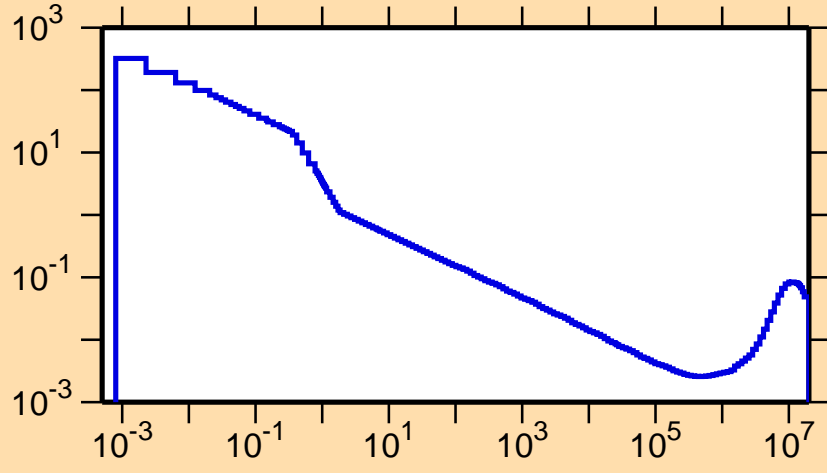
\sigma vs. E for ^{130}\text{Sm}(n,\alpha)
