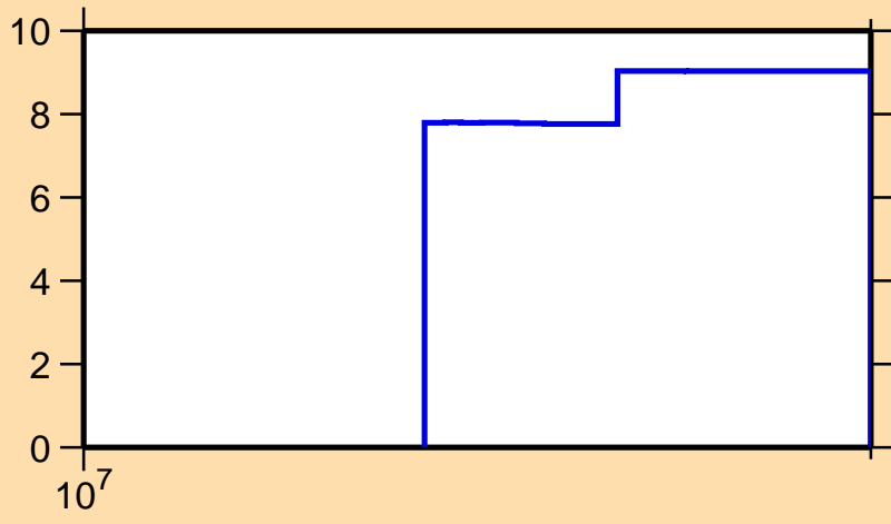
\Delta\sigma/\sigma vs. E for ^{130}\text{Sm}(n,\text{el.})
