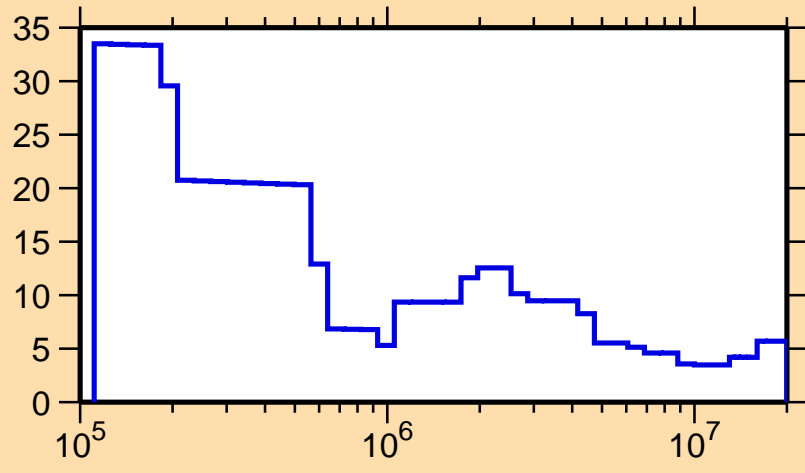
\Delta\sigma/\sigma vs. E for ^{130}\text{Sm}(n,\text{tot.})
