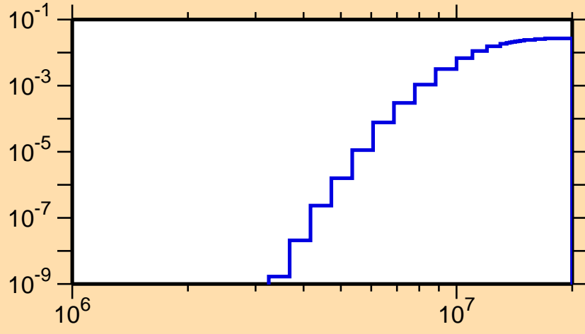
\sigma vs. E for ^{131}\text{Sm}(n,d)
