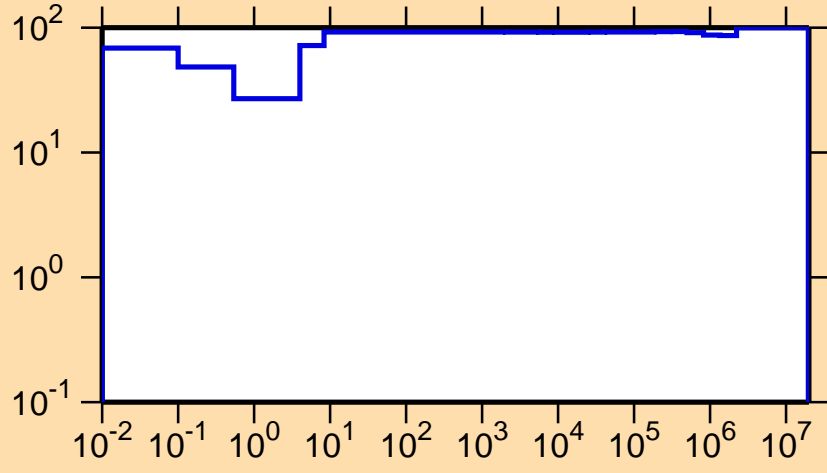
\Delta\sigma/\sigma vs. E for ^{131}\text{Sm}(n,\gamma)
