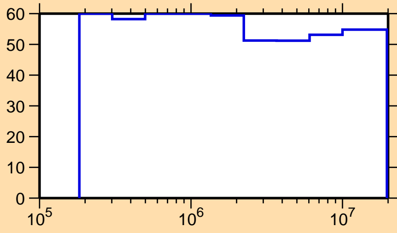
\Delta\sigma/\sigma vs. E for ^{131}\text{Sm}(n,\text{inel.})
