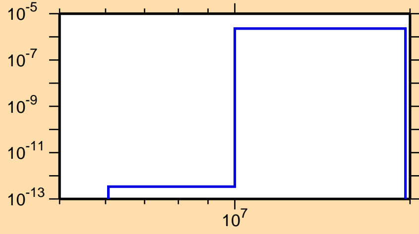
\sigma vs. E for ^{131}\text{Sm} (mt 45)
