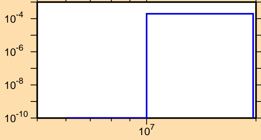
\sigma vs. E for ^{131}\text{Sm}(n,t)
