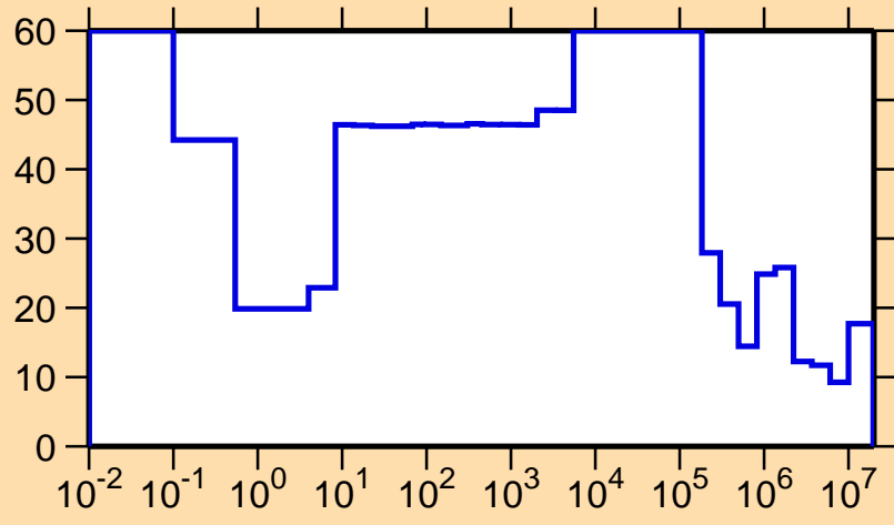
\Delta\sigma/\sigma vs. E for ^{131}\text{Sm}(n,\text{tot.})
