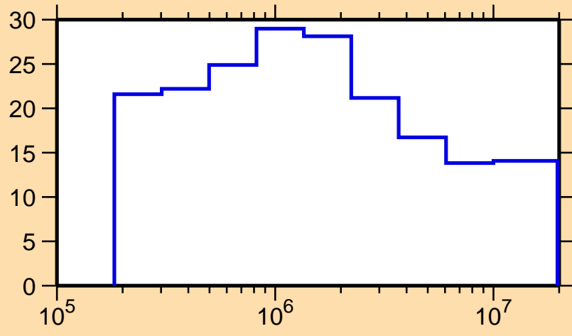
\Delta\sigma/\sigma vs. E for ^{131}\text{Sm}(n,\text{nonel.})
