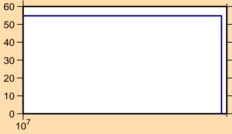
\Delta\sigma/\sigma vs. E for ^{131}\text{Sm}(n,\text{inel.})
