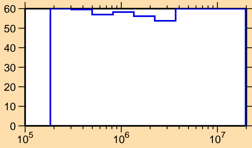
\Delta\sigma/\sigma vs. E for ^{131}\text{Sm}(n,n_1)
