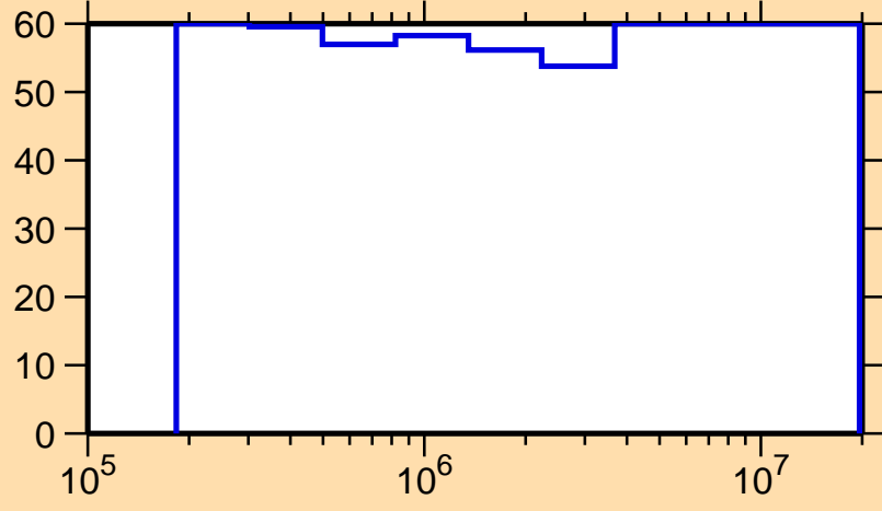
\Delta\sigma/\sigma vs. E for ^{131}\text{Sm}(n,n_1)
