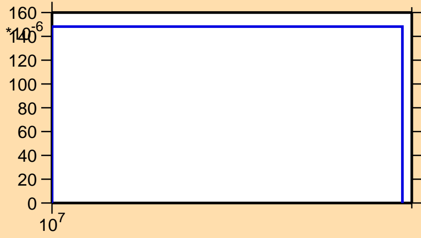
\sigma vs. E for ^{131}\text{Sm}(n,2n)
