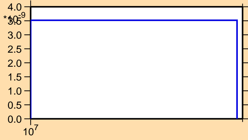
\sigma vs. E for ^{131}\text{Sm}(n,\text{nd})
