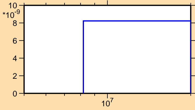
\sigma vs. E for ^{131}\text{Sm}(\text{mt117})
