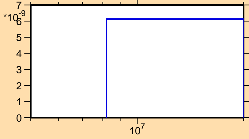
\sigma vs. E for ^{131}\text{Sm} (mt 34)
