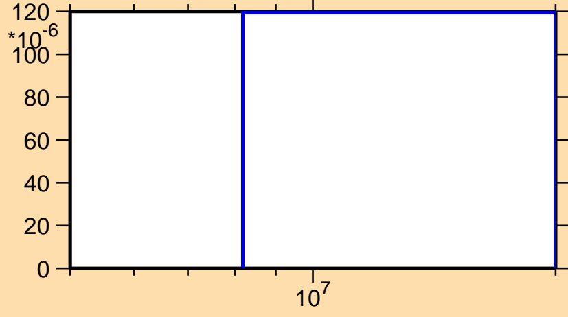
\sigma vs. E for ^{131}\text{Sm}(n,2n)
