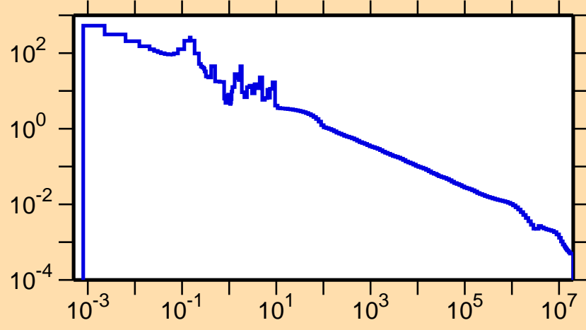
\sigma vs. E for ^{133}\text{Sm}(n,\gamma)
