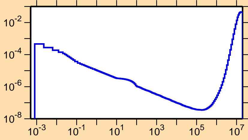
\sigma vs. E for ^{133}\text{Sm}(n,p\alpha)
