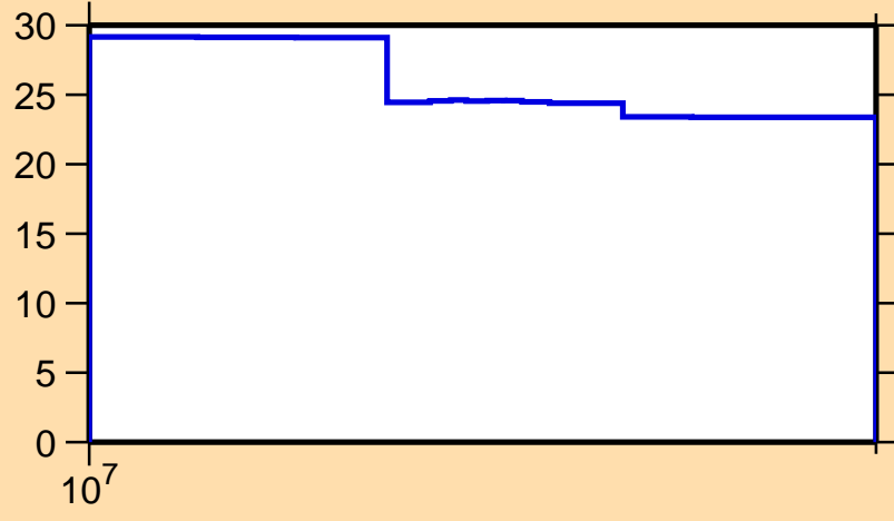
\Delta\sigma/\sigma vs. E for ^{133}\text{Sm}(n,\text{el.})
