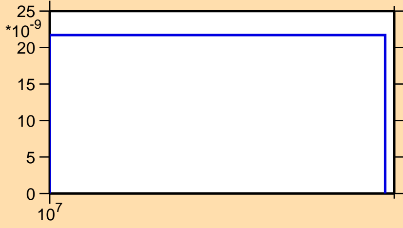
\sigma vs. E for ^{133}\text{Sm}(n,\text{nd})
