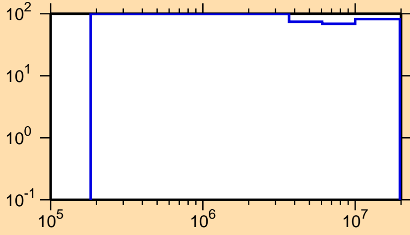
\Delta\sigma/\sigma vs. E for ^{133}\text{Sm}(n,n\text{cont.})
