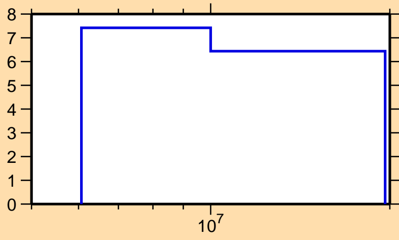
\Delta\sigma/\sigma vs. E for ^{133}\text{Sm}(n,\text{nonel.})
