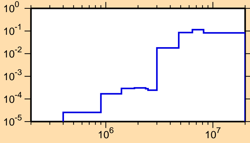
\sigma vs. E for ^{133}\text{Sm}(n,n\text{cont.})
