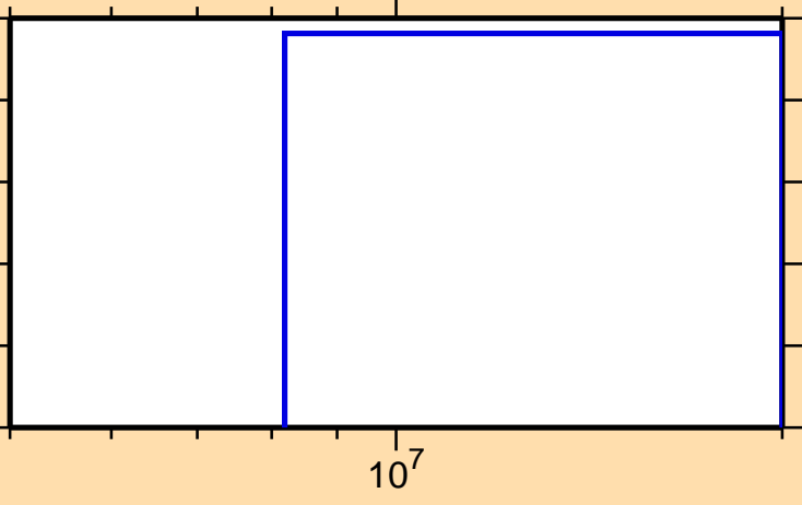
\sigma vs. E for ^{133}\text{Sm} (mt 45)
