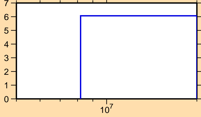
\Delta\sigma/\sigma vs. E for ^{133}\text{Sm}(n,\text{el.})
