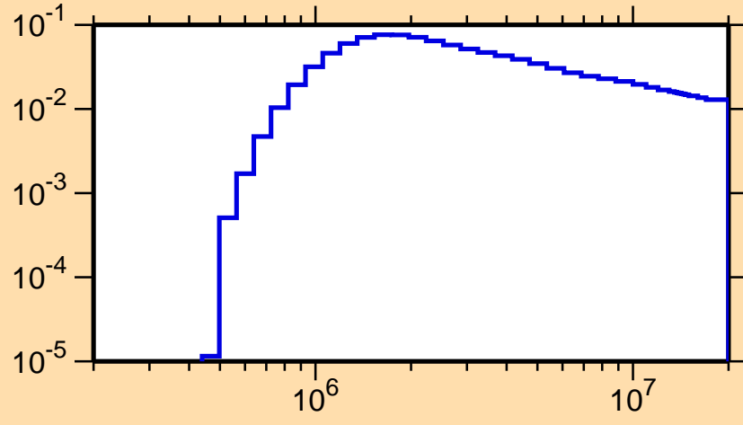
\sigma vs. E for ^{134}\text{Sm}(n,n_2)
