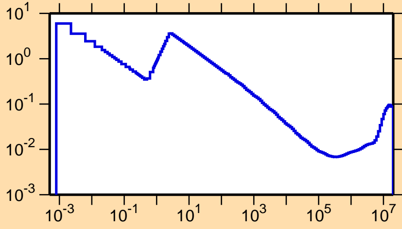
\sigma vs. E for ^{134}\text{Sm}(n,\alpha)
