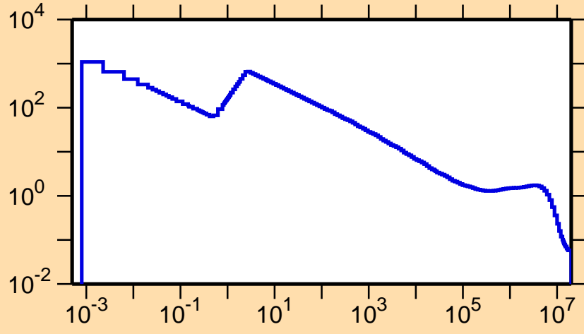
\sigma vs. E for ^{134}\text{Sm}(n,p)
