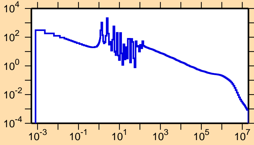
\sigma vs. E for ^{134}\text{Sm}(n,\gamma)
