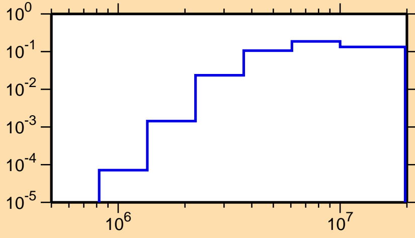
\sigma vs. E for ^{134}\text{Sm}(n,n\text{cont.})
