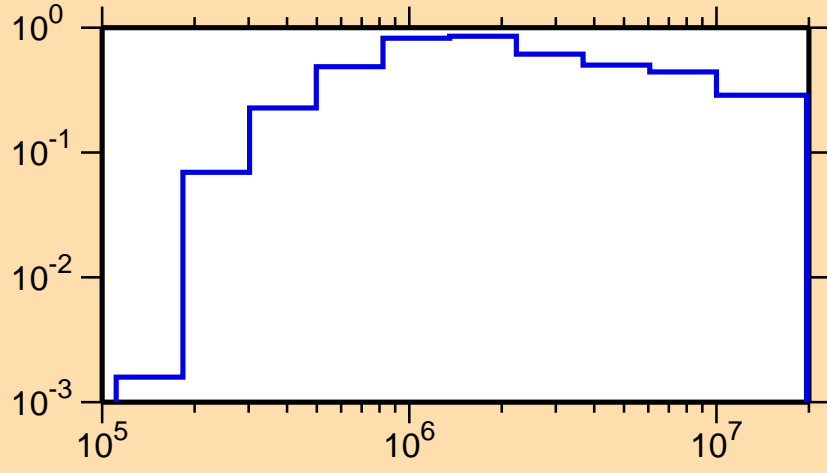
\sigma vs. E for ^{134}\text{Sm}(n,\text{inel.})
