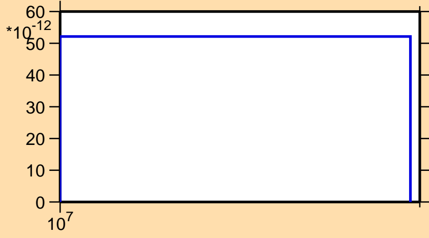
\sigma vs. E for ^{134}\text{Sm}(n,2n\alpha)
