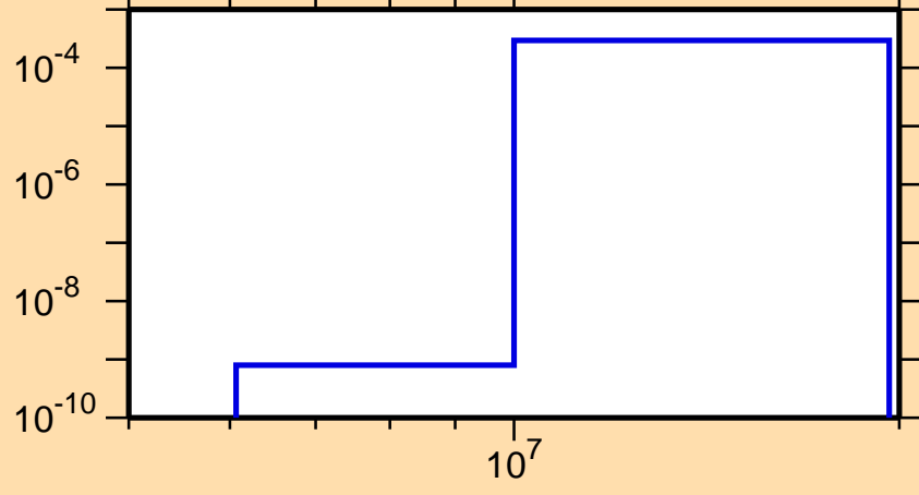
\sigma vs. E for ^{134}\text{Sm}(n,pd)
