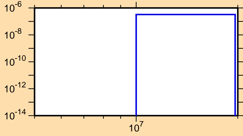
\sigma vs. E for ^{134}\text{Sm} (mt 45)
