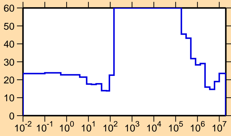
\Delta\sigma/\sigma vs. E for ^{134}\text{Sm}(n,el.)
