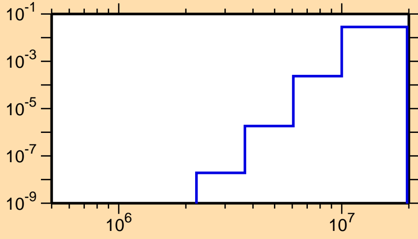
\sigma vs. E for ^{134}\text{Sm}(n,p\alpha)
