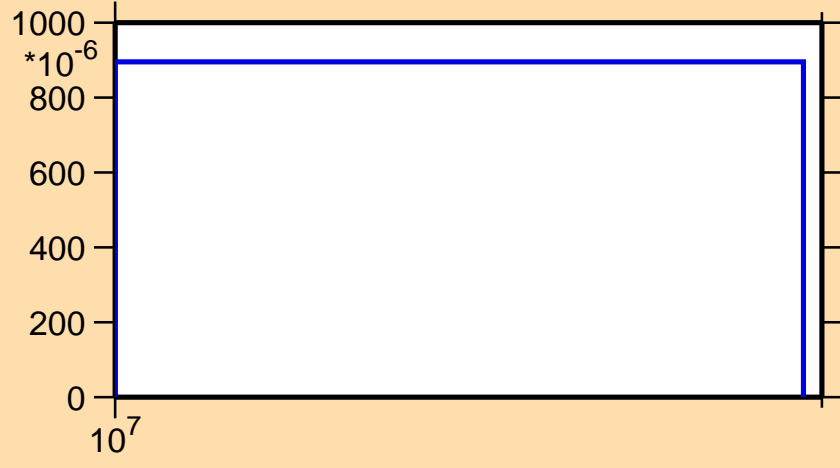
\sigma vs. E for ^{134}\text{Sm}(n,2n)
