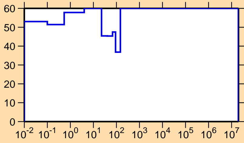
\Delta\sigma/\sigma vs. E for ^{134}\text{Sm}(n,\gamma)
