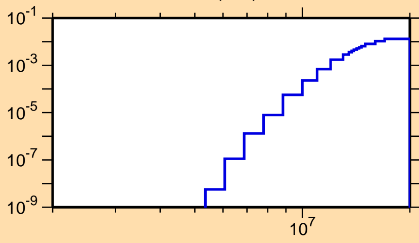
\sigma vs. E for ^{136}\text{Sm}(n,d)
