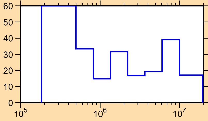
\Delta\sigma/\sigma vs. E for ^{136}\text{Sm}(n,\text{el.})
