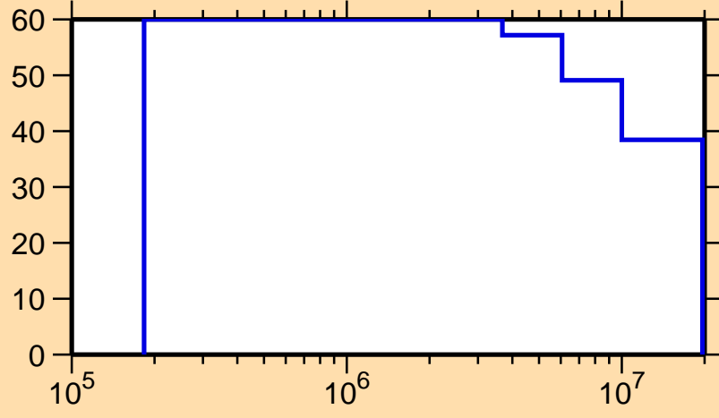
\Delta\sigma/\sigma vs. E for ^{136}\text{Sm}(n,n_1)
