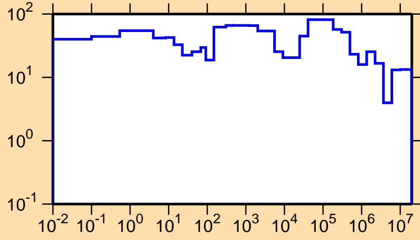
\Delta\sigma/\sigma vs. E for ^{136}\text{Sm}(n,\text{tot.})
