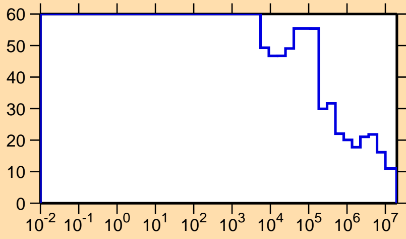
\Delta\sigma/\sigma vs. E for ^{136}\text{Sm}(n,\text{nonel.})
