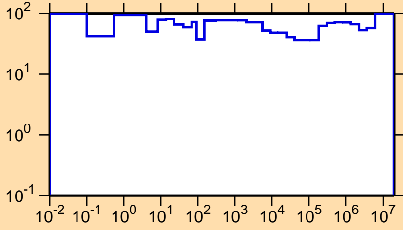
\Delta\sigma/\sigma vs. E for ^{136}\text{Sm}(n,\gamma)
