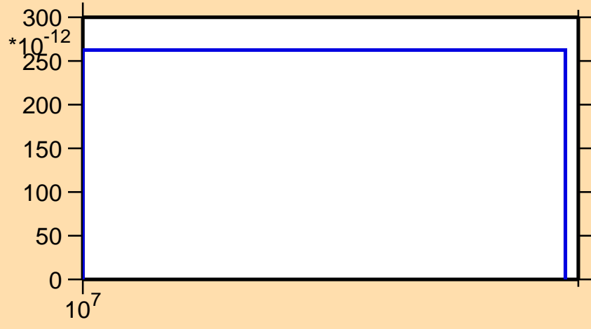
\sigma vs. E for ^{136}\text{Sm}(n,\text{nd})
