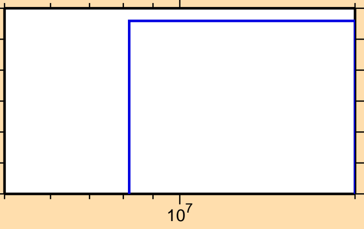
\sigma vs. E for ^{136}\text{Sm} (mt 45)
