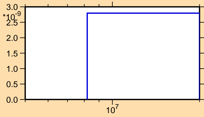
\sigma vs. E for ^{136}\text{Sm}(n,\text{pt})
