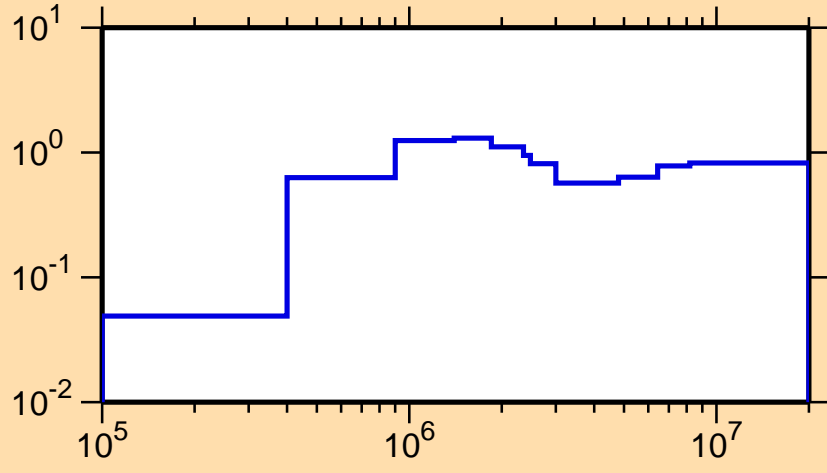
\sigma vs. E for ^{136}\text{Sm}(n,\text{inel.})
