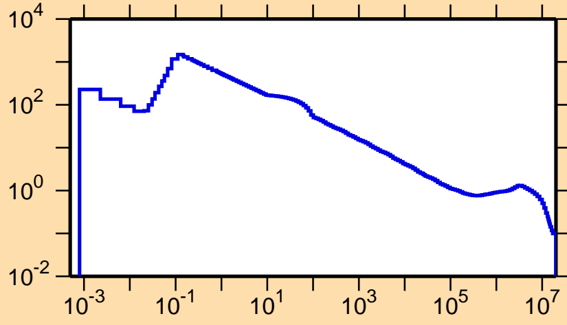
\sigma vs. E for ^{137}\text{Sm}(n,p)
