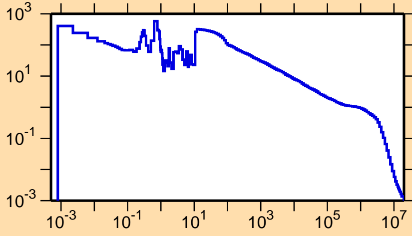
\sigma vs. E for ^{137}\text{Sm}(n,\gamma)
