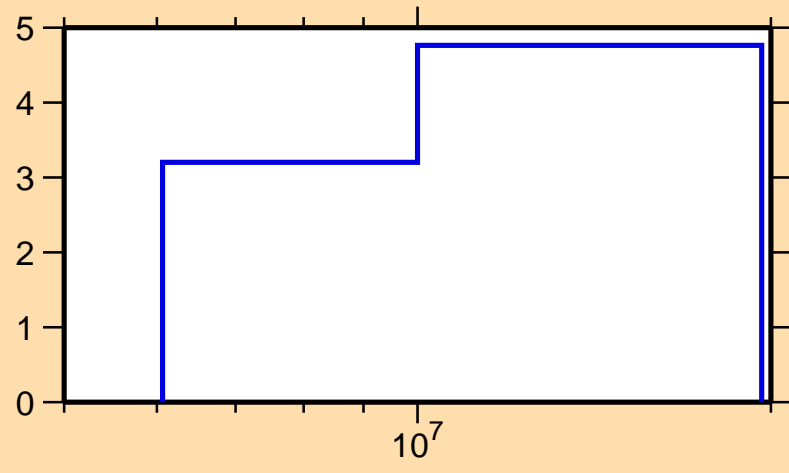
\Delta\sigma/\sigma vs. E for ^{137}\text{Sm}(n,\text{el.})
