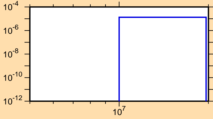
\sigma vs. E for ^{137}\text{Sm}(n,pd)
