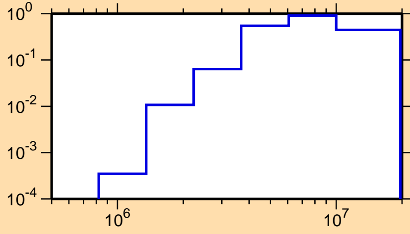
\sigma vs. E for ^{137}\text{Sm}(n,n\text{cont.})
