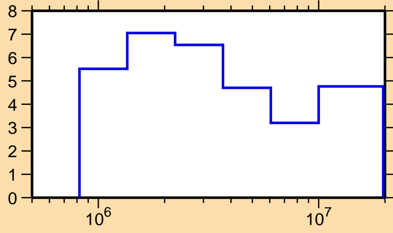
\Delta\sigma/\sigma vs. E for ^{137}\text{Sm}(n, el.)
