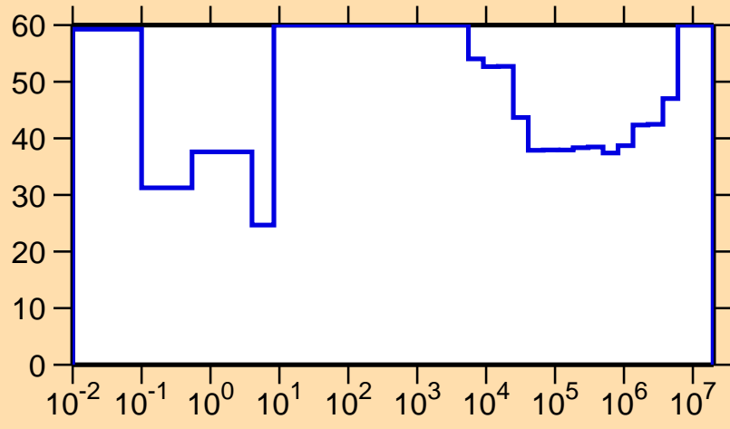
\Delta\sigma/\sigma vs. E for ^{137}\text{Sm}(n,\gamma)
